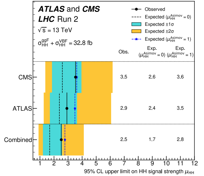
FIG. 2. Expected and observed 95% CL upper limits on the total HH signal strength, defined as the ratio of the measured cross section to the sum of the ggF and VBF HH SM cross sections, for ATLAS, CMS, and the combination from both experiments. The median expected limits on \mu_{HH} are obtained under the hypotheses of no HH signal ( \mu_{HH}^{\text{Asimov}} = 0 ) or assuming the presence of the SM HH signal ( \mu_{HH}^{\text{Asimov}} = 1 ). The \pm 1\sigma and \pm 2\sigma bands are computed under the \mu_{HH}^{\text{Asimov}} = 0 hypothesis.
