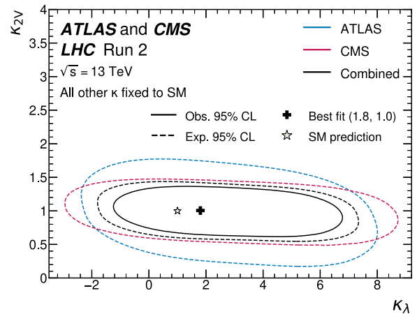
FIG. 4. Observed and expected 95% CL contours for the simultaneous scan of the profile likelihood as a function of \kappa_\lambda and \kappa_{2V} . The expected constraints from the individual experiments are also shown. All the other Higgs boson couplings are fixed to their SM predictions.
