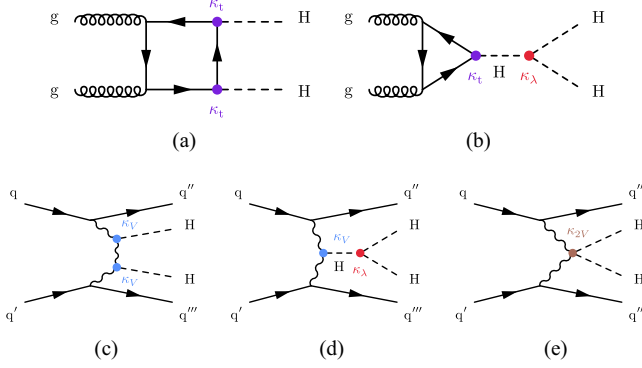
FIG. 1. Leading order Feynman diagrams for (a),(b) ggF and (c)–(e) VBF HH production. The Higgs boson coupling modifiers are indicated on the relevant vertices: in (b) and (d) the trilinear Higgs boson self coupling modifier \kappa_\lambda , in (e) the quartic VVHH coupling modifier \kappa_{2V} , in (a) and (b) the top Yukawa coupling modifier k_t , and in (c) and (d) the VVH coupling modifier \kappa_V .
