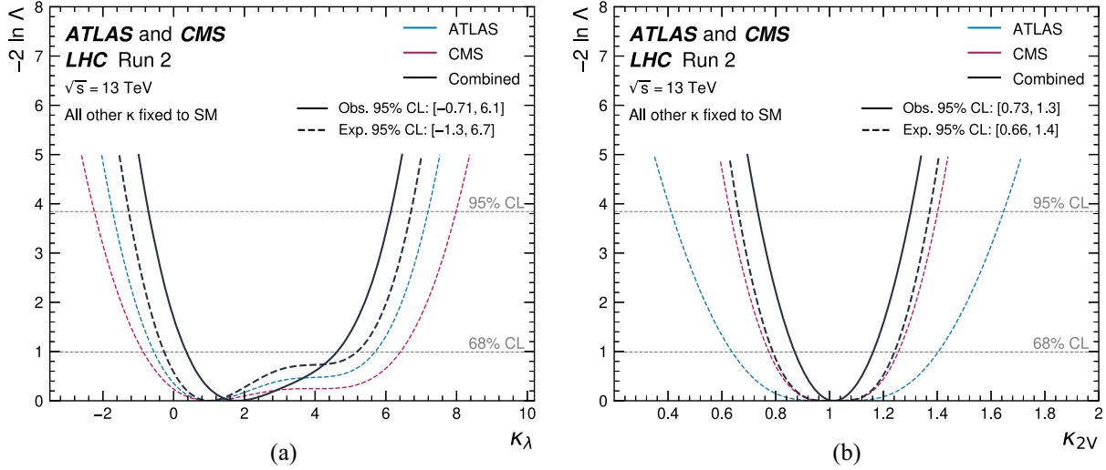
FIG. 3. Expected negative log-likelihood ( -2 \ln \Delta ) values as functions of (a) \kappa_\lambda and (b) \kappa_{2V} for ATLAS, CMS, and the expected and observed values for the combination from both experiments. All the other Higgs boson couplings are fixed to their SM predictions.
