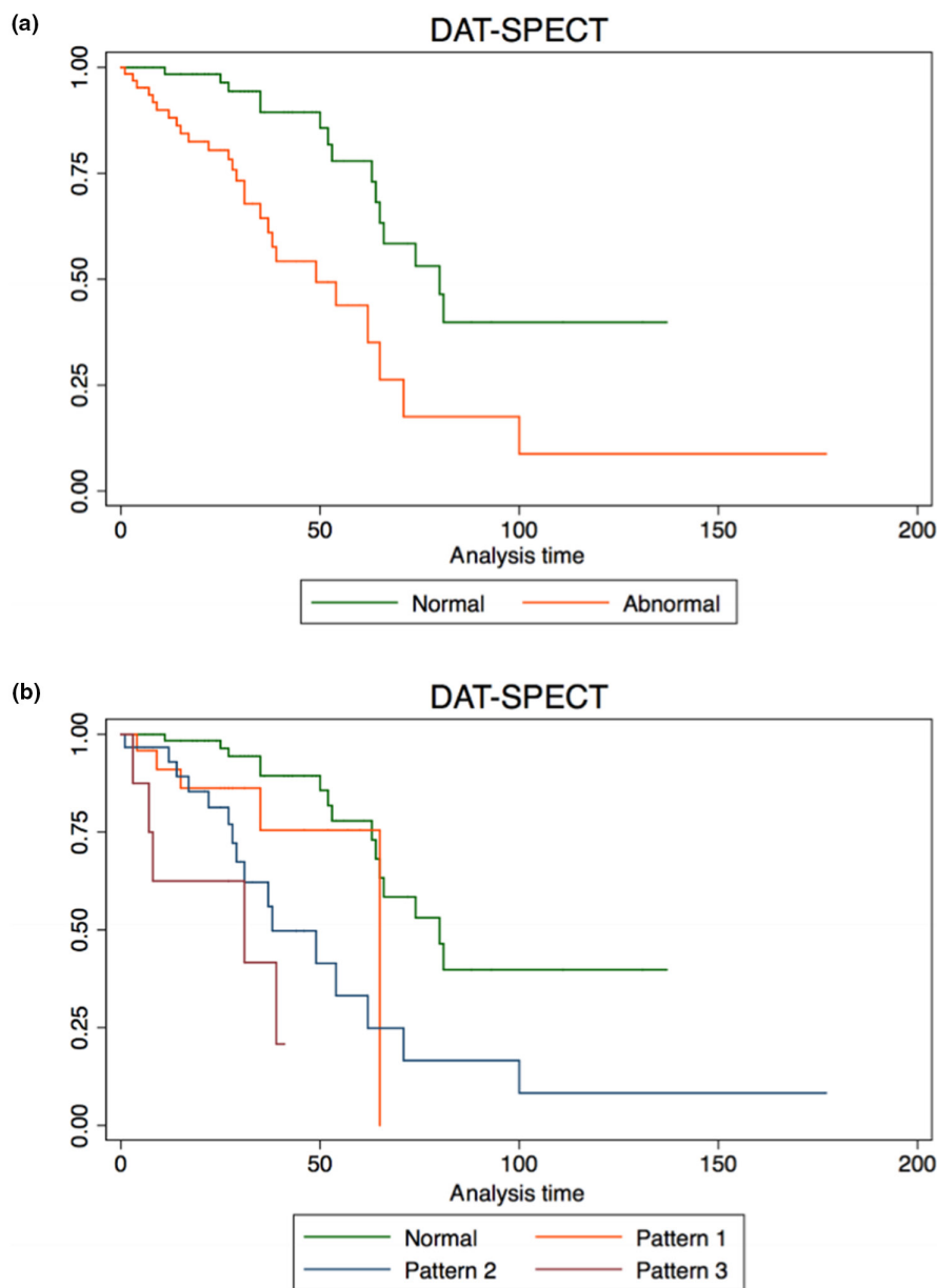
FIGURE 2 Kaplan–Meier analysis: [ ^{123}\text{I} ]-FP-CIT-SPECT (123-radiolabeled 2 \beta -carbomethoxy-3 \beta -(4-iodophenyl)-N-(3-fluoropropyl)-nortropane-single positron emission computed tomography). (a) The dichotomic normal/abnormal classification is shown. (b) When a semi-quantitative categorization is used, a survival gradient from normal to pattern 3 can be noticed. Pattern 1 is more similar to normal, pattern 2 is more similar to pattern 3. [Colour figure can be viewed at wileyonlinelibrary.com ]
