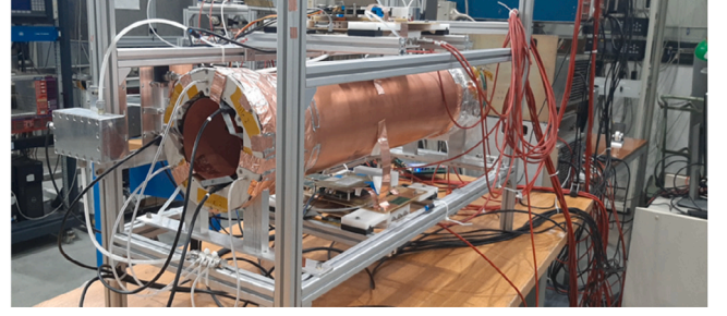
Fig. 3. The cylindrical \mu -RWELL.
