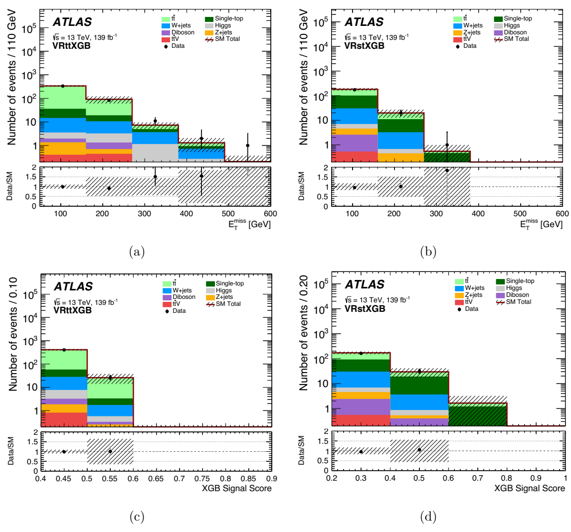
Figure 7. Post-fit E_T^{\text{miss}} and signal output score distributions: (a) and (c) in t\bar{t} , (b) and (d) in single-top VRs. The uncertainty bands plotted include all statistical and systematic uncertainties. The overflow events, where present, are included in the last bin. The lower panels of the plots show the ratio of the observed data to the total background prediction.
