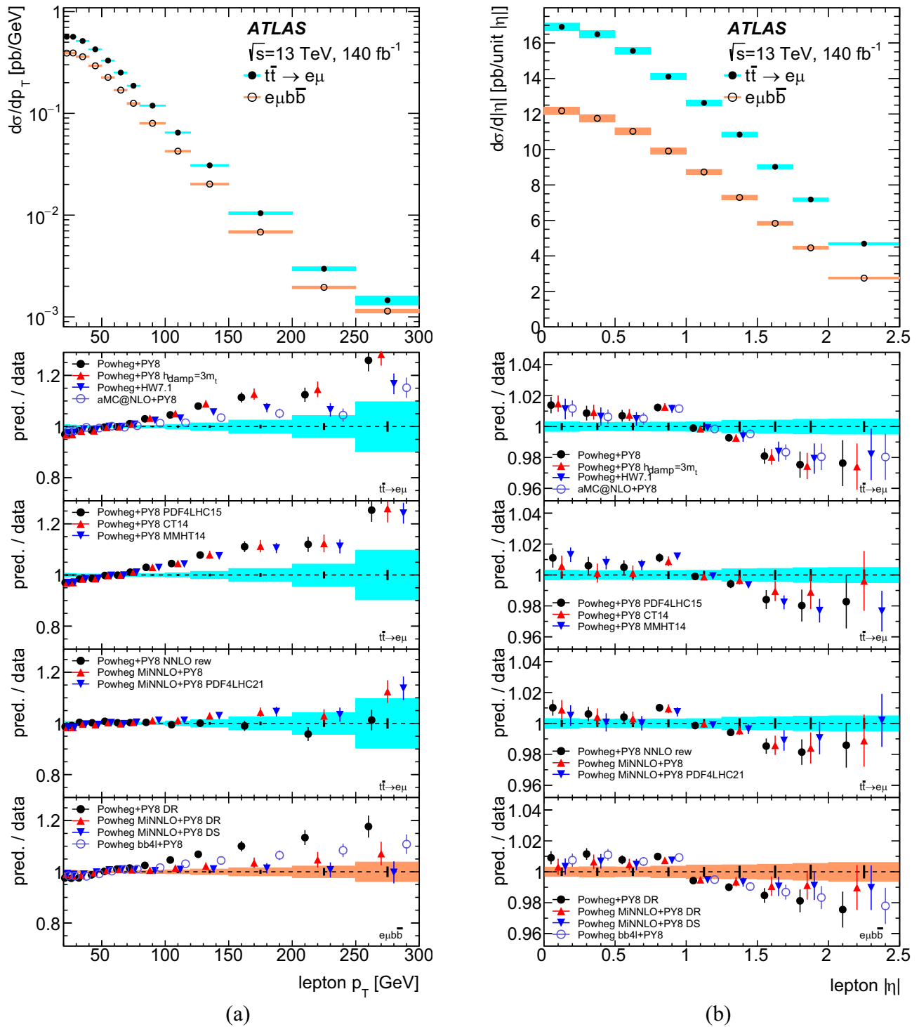
Fig. 12 Differential cross-sections as functions of (a) p_T^\ell and (b) |\eta^\ell| . The upper panels show the measured absolute t\bar{t} \rightarrow e\mu (filled points) and e\mu b\bar{b} (open points) cross-sections, including the contributions from W \rightarrow \tau \rightarrow e/\mu decays, with the total uncertainties shown by the shaded bands. The other panels show ratios of various predictions to the measured normalised differential cross-sections, for t\bar{t} \rightarrow e\mu (mid-
