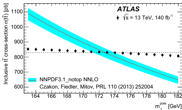
Fig. 11 The red line shows the predicted inclusive t\bar{t} cross-section at \sqrt{s} = 13 TeV as a function of m_t^{\text{pole}} for the NNP3.1_notop PDF set, with the cyan band indicating the total uncertainty in the prediction from PDF+ \alpha_s and QCD scale uncertainties. The black points show the experimental measurement with its uncertainty and dependence on the assumed value of m_t through acceptance and background corrections. The dotted line shows the experimental central value at a fixed top quark mass of 172.5 GeV
