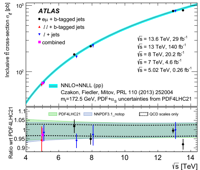
Fig. 10 The upper panel shows the inclusive t\bar{t} cross-section as a function of centre-of-mass energy \sqrt{s} , comparing ATLAS results from the e\mu , dilepton ( \ell\ell ) and lepton+jets final states (and the combination of \ell\ell and lepton+jets at \sqrt{s} = 5.02 TeV) with NNLO+NNLL theoretical predictions [6,21] using the PDF4LHC21 PDF set [22]. The lower panel shows the ratios of measurements and predictions to the central value of the prediction with PDF4LHC21. The total uncertainties when using the PDF4LHC21 and NNPDF3.1_notop PDF sets are shown as the overlapping coloured bands, and the dotted lines show the QCD scale uncertainties alone
