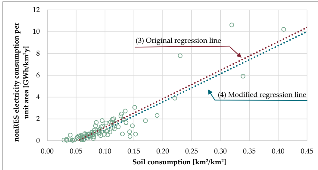
Figure 9. Soil consumption per unit area versus non-RES electricity consumption per unit of surface.
