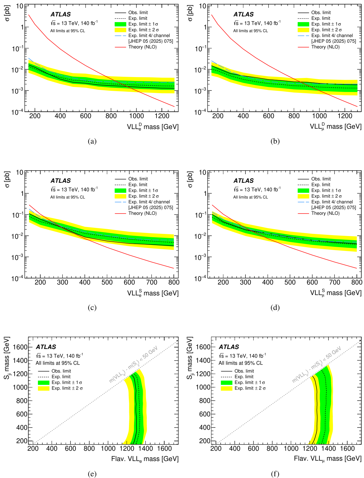
Fig. 10 Combined observed and expected limits at 95% CL on the cross-section ( \sigma ) as a function of the VLL mass for the a VLL_e^D , b VLL_\mu^D , c VLL_e^S , d VLL_\mu^S models, and on the plane of the S_{ji} mass versus the VLL mass for the e flavourful VLL_e , and f flavourful VLL_\mu
