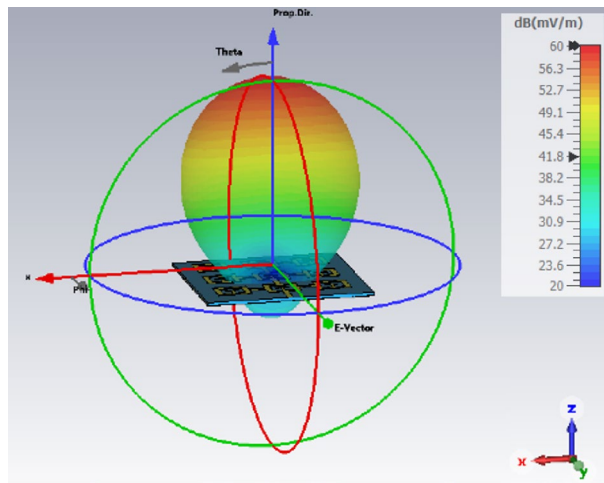
Figure 9. Simulated radiation pattern of the single antenna array.
