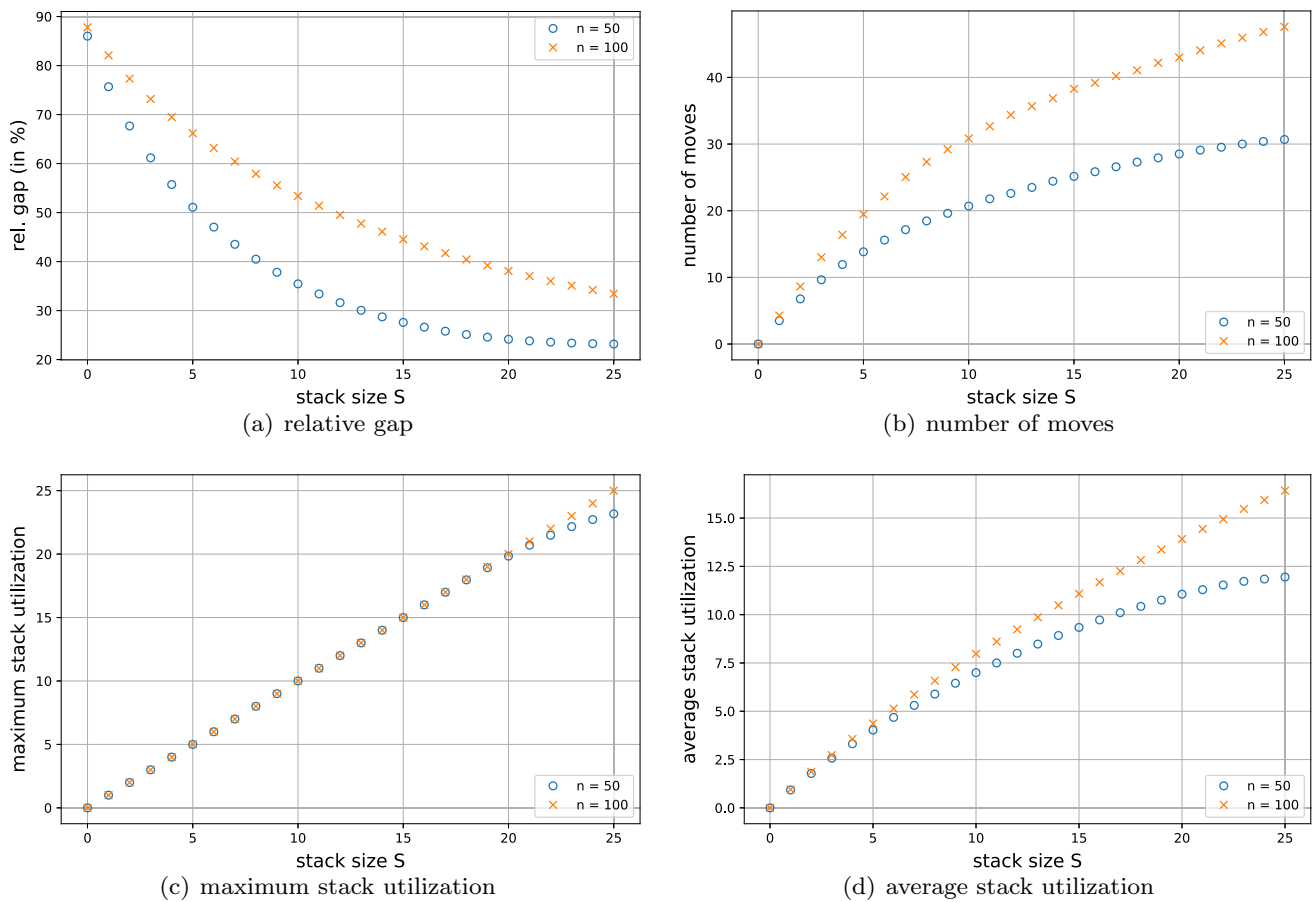
Fig. 3 Effect of increasing stack size S for 1|\text{resch-LIFO}|\sum w_j C_j
