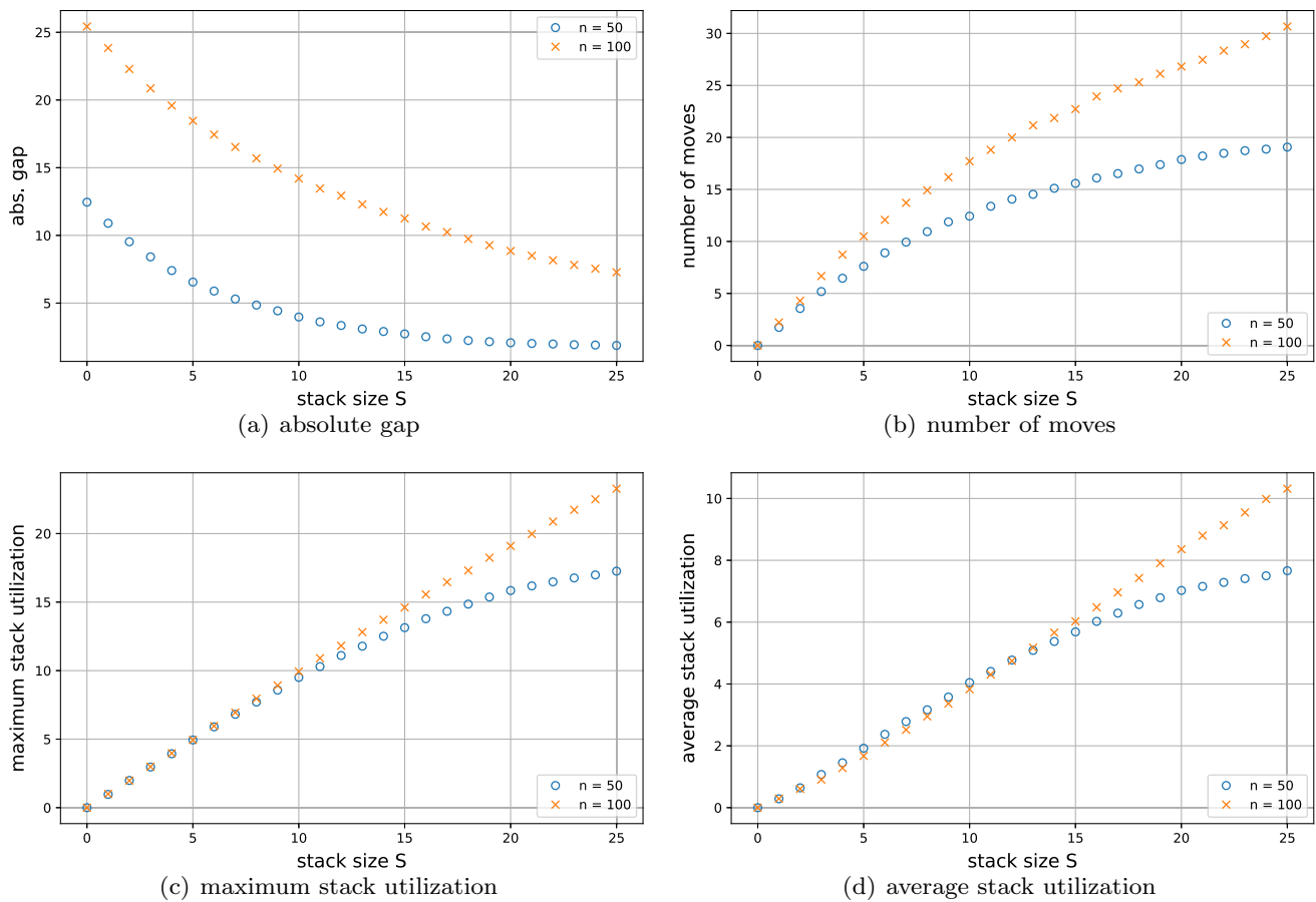
Fig. 5 Effect of increasing stack size S for |\text{resch-LIFO}| \sum U_j
