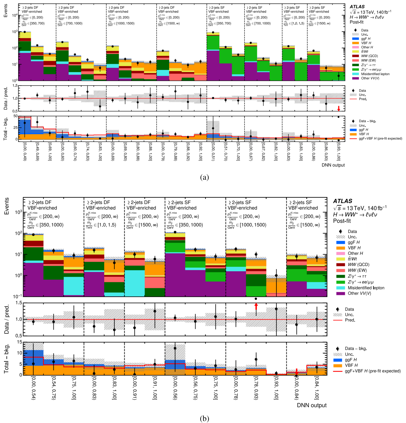
Fig. 9 Post-fit DNN distributions in the VBF \geq 2-jets a low and b high p_T^{\ell, \text{miss}} SRs entering the STXS measurement for both the DF and SF channels; the post-fit results are obtained from the 15-POI fit. The vertical dashed lines delineate different SRs. The middle panels show the ratios of the data to the sum of the fitted signal and background, and the bottom panels show the differences between
