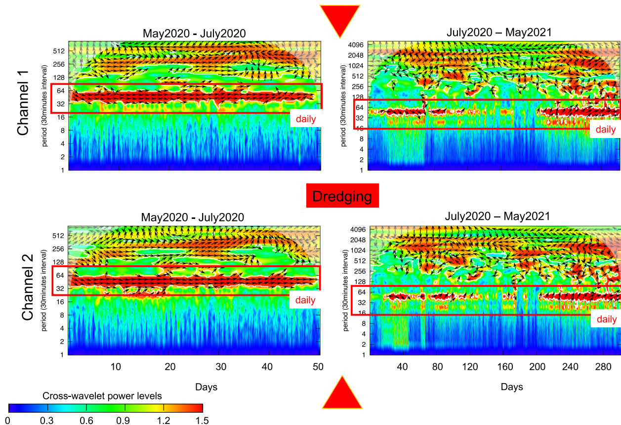
Fig. 3. Cross-wavelet transformation of detrended oxygen and temperature time-series data. The x-axis represents time (in days), while the y-axis represents the periodicity (in half hours). Cross-wavelet power quantifies the relative contribution of variation in water oxygen and temperature at each period to the total variance over time. High power is represented by warm colours and low power is represented by cool colours. Black contours designate regions of significantly high temporal variation compared to a null model (red noise). Values outside of the cone of influence—the bolder colour cone shape—are less reliable due to edge effects. Thick contour indicates the 5 % significance level against red noise. Arrows indicate the time-series relative phase (pointing left: the two time-series are in antiphase; pointing right: in-phase). Red boxes highlight the significant periodicity of co-variation of oxygen and temperature.
