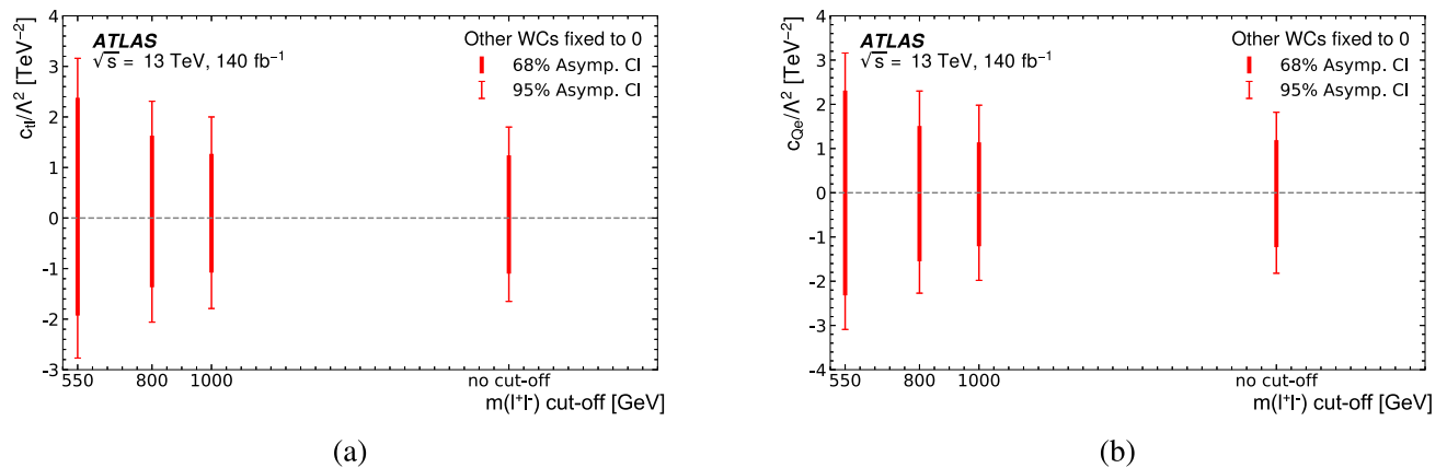
Fig. 7 The confidence intervals for a c_{tl} and b c_{Qe} from fits to data for different values of the m(\ell^+\ell^-) upper cut-off. The results use the asymptotic assumption to calculate the intervals (Asymp.)
