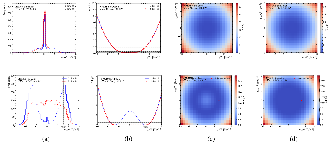
Fig. 9 Studies on the sensitivity to multiple WCs at a time. Results are shown for fits considering only the statistical uncertainties for the SM expectation, for (top) all WCs = 0, and (bottom) for an injected value of c_{tl} = 1.53 , close to the 95% confidence interval limit. The distributions
