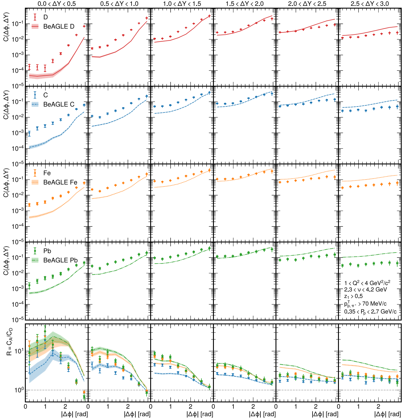
Fig. 2. Correlation functions for D, C, Fe, and Pb (from top to bottom, first four rows), with \Delta\phi on the x axis within each panel and different bins of \Delta Y for each column. These are compared to calculations from the BeAGLE model [9] (curves). The horizontal caps in the error bars represent the systematic uncertainties, while the outer bars represent the total systematic and statistical uncertainty (added in quadrature). Bottom row: same for the ratios between the nuclear and deuterium correlation functions.
