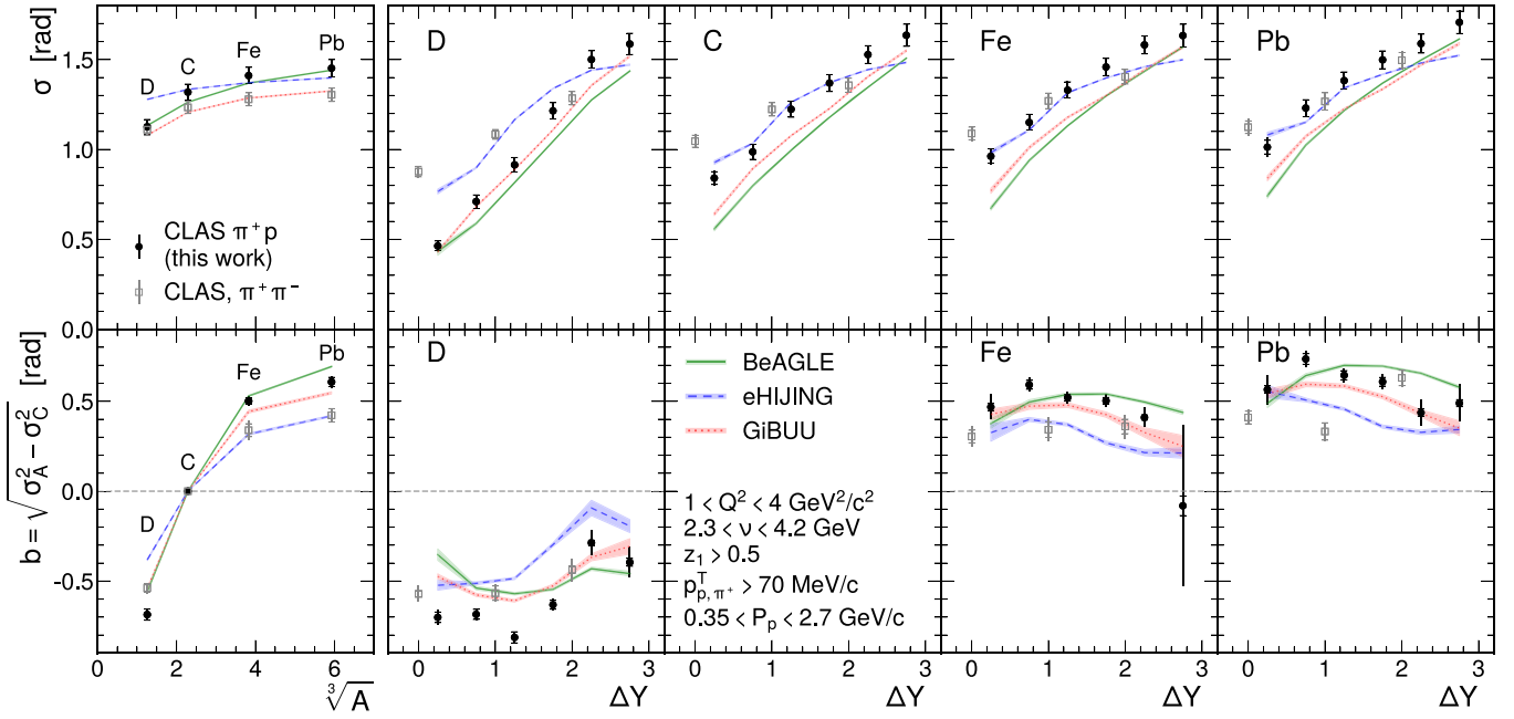
Fig. 3. Top row: RMS width \sigma as a function of \sqrt{A} (left-most panel), and as a function of \Delta Y for each target (other panels). Bottom row: same for the azimuthal broadening, b . The horizontal caps in the error bars represent the systematic uncertainties, while the outer bars represent the total systematic and statistical uncertainty (added in quadrature). The results are compared to the predictions from the BeAGLE [9], eHIJING [41], and GiBUU [42] models, as well as analogous measurements of the dipion channel from Ref. [20] (gray, open squares). The broadenings for the dipion channel were reported in Ref. [20] with respect to deuterium, and have been re-calculated with respect to carbon in order to compare them to the results of this work.
