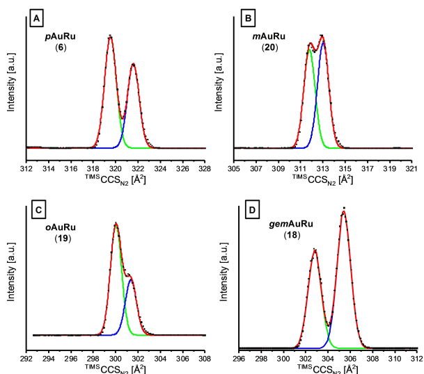
Figure 6. Mobilograms of the AuRu isomers obtained from IMS.
