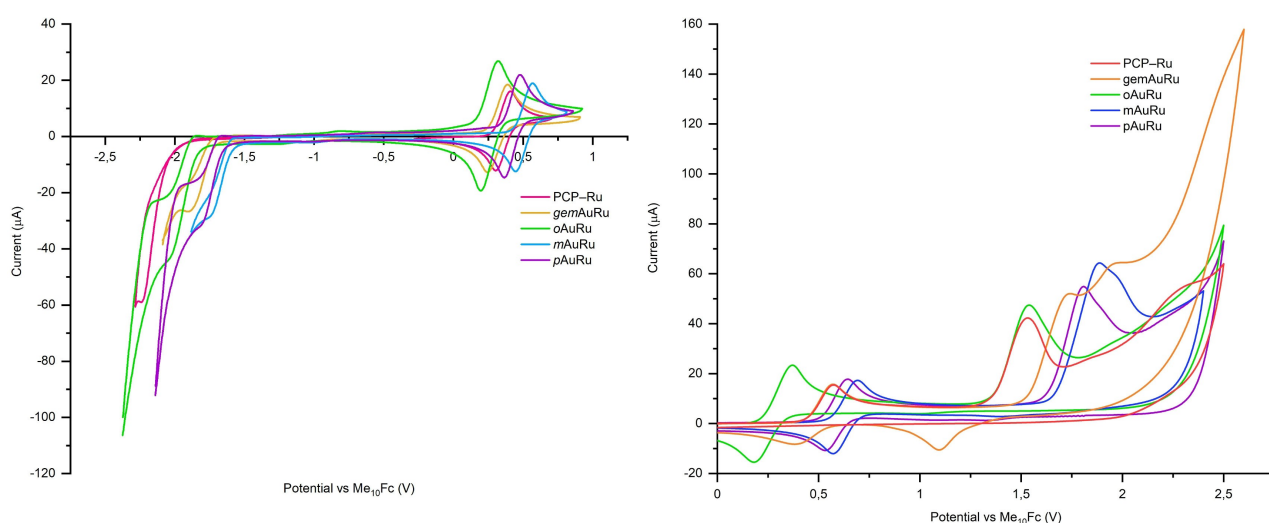
Figure 11. Cyclic voltammograms of PCP-Ru ( 22 ) and AuRu isomers 6 and 18–20 (left) and CV spectra of the second oxidation process (right) ( 0.1 M ^t\text{Bu}_4\text{NPF}_6 , \text{CH}_2\text{Cl}_2 , 100 mV/s).
