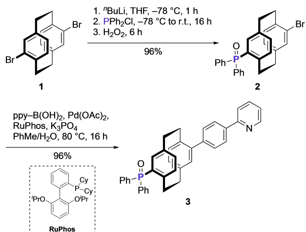
Scheme 1. Selective mono lithiation followed by Suzuki-Miyaura reaction to obtain the intermediate ligand structure 3. ppy = 2-phenylpyridine.
