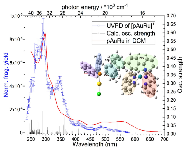
Figure 10. Gas phase UV-PD spectrum (blue) and calculated transitions (stick) of [\text{pAuRu}]^+ calculated with B3LYP, as well as the liquid phase absorption spectrum in \text{CH}_2\text{Cl}_2 (red) of \text{pAuRu} ( 6 ). The different ligands of the complex are marked with their abbreviations.
