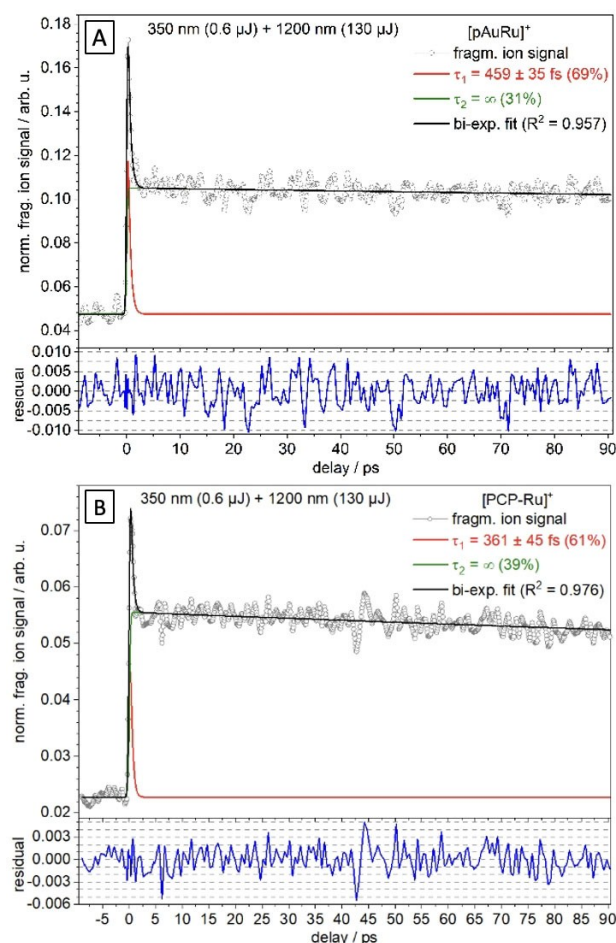
Figure 13. Normalized transient fragment ion intensity of [ p AuRu] + (A) and [PCP-Ru] + (B) recorded at \lambda_{\text{pump}} = 350 nm on a 100 ps time window; bi-exponential fit (black) is given along with the fit decomposition (green and red). Fit residual is shown below (blue).
