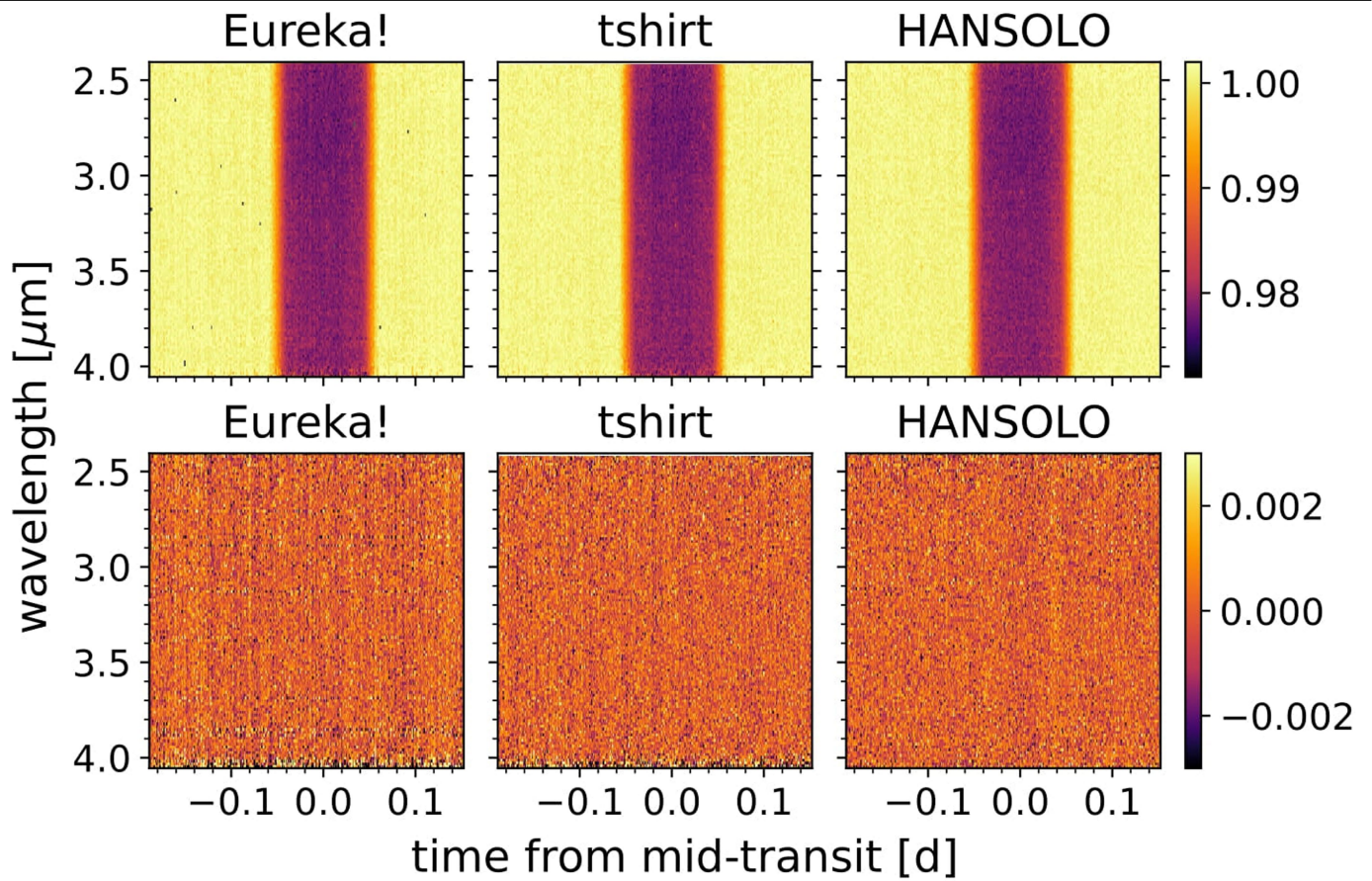
Extended Data Fig. 6 | JWST's NIRCam data of WASP-39 as a function of time and wavelength for each independent reduction (top) and their residuals (bottom). Top: time-series NIRCam data for the WASP-39b system, from three
