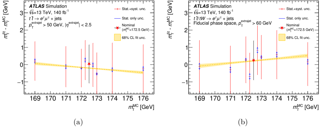
Figure 5. Difference between the extracted m_t^{\text{fit}} value in the \chi^2 fit and the mass value m_t^{\text{MC}} in the POWHEG+PYTHIA 8 t\bar{t} simulations, (a) for the 2 \rightarrow 3 and (b) 2 \rightarrow 7 measurements. Each point corresponds to a mass value extracted using the parameterized mass dependence of the parton-level distributions obtained from the simulated MC samples, with the inner uncertainty bars representing the statistical uncertainties due to the limited size of the simulated samples and the outer bars representing the total experimental uncertainty associated with that measurement. A linear fit is performed across the various mass points, considering only their fully uncorrelated statistical uncertainties. Another uncorrelated effect, which originates from the interplay of statistical and systematic effects in the covariance matrices, further scatters the fitted mass values and is not considered in the linear fit. The 68% confidence level (CL) associated with the fit is shown with a filled area. The 172.5 GeV mass point is not included among the fitted points.
