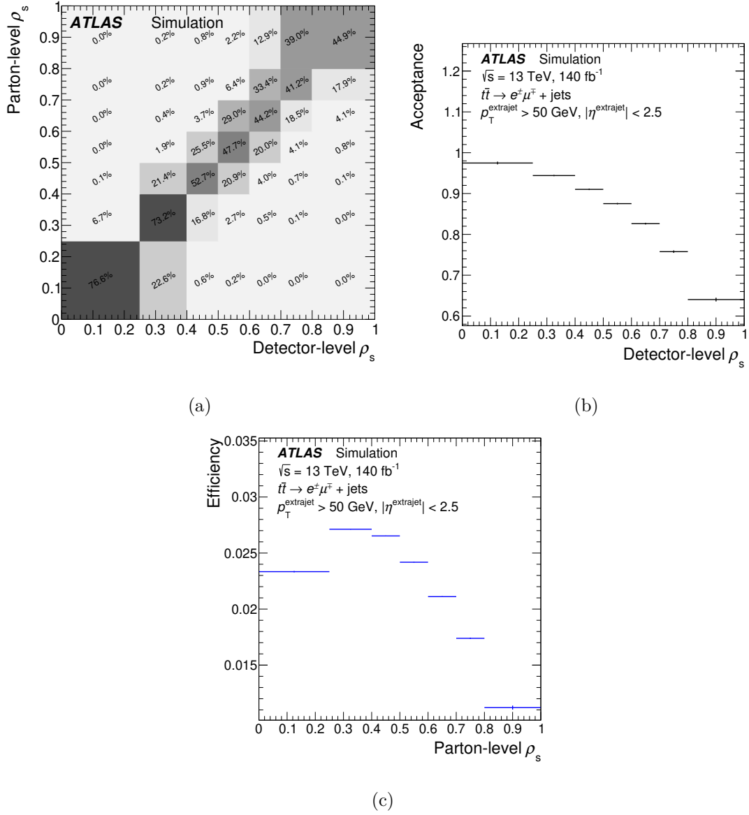
Figure 3. The (a) migration matrix and (b) the acceptance and (c) efficiency factors for events considered in the unfolding to the 2 \rightarrow 3 parton level. The matrix and correction factors are built from the nominal simulation of t\bar{t} + 1\text{-jet} events using the POWHEG+PYTHIA 8 generator. Vertical bars represent MC statistical uncertainties.
