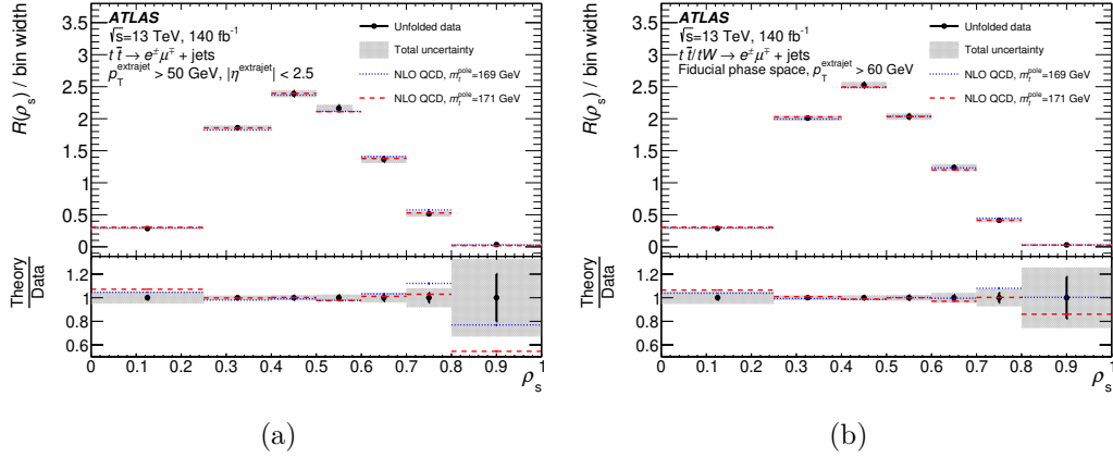
Figure 4. The measured normalized differential cross-section \mathcal{R}(\rho_s; m_t^{\text{pole}}) unfolded to (a) the 2 \rightarrow 3 parton level and (b) the 2 \rightarrow 7 parton level. The error bars on the marker indicate the statistical uncertainty, the gray band the total experimental uncertainty. Theoretical predictions at fixed-order NLO QCD for m_t^{\text{pole}} = 169 GeV (dotted line) and m_t^{\text{pole}} = 171 GeV (dashed line) are also shown, without their associated uncertainties.
