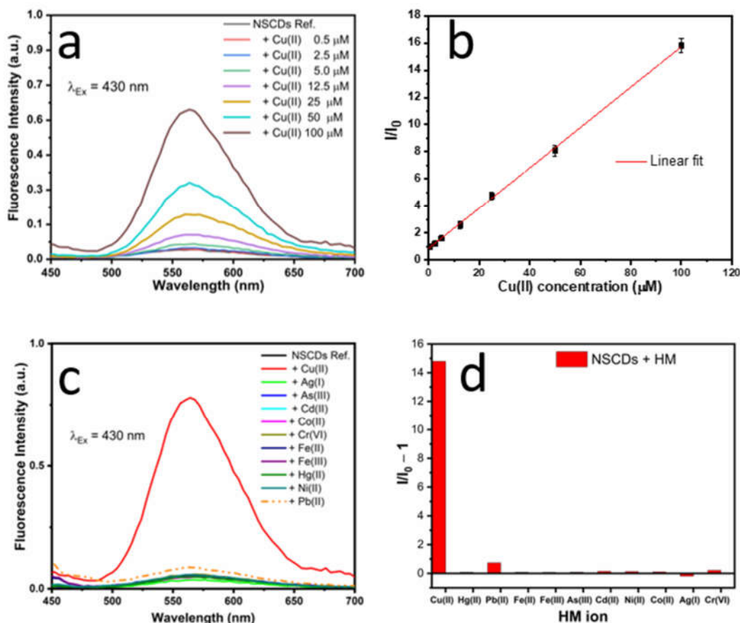
Figure 6. (a) Emission spectra of NSCDs in the presence of Cu(II) at different concentrations. (b) calibration plot showing the fluorescence enhancement intensity vs. the Cu(II) concentration over
