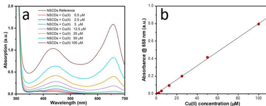
Figure 4. (a) UV–Vis absorption spectra of NSCDs-sensing solution upon the addition of Cu(II) ions at different concentrations; (b) calibration curve.
