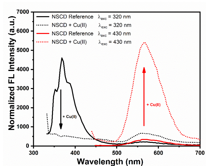
Figure 5. Variation of fluorescence emission of NSCD sensing solution excited at 320 nm (black curve) or 430 nm (red) upon the addition of 100 μM Cu(II).
