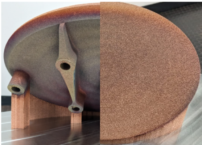
Figure 18. Side view of upper and equatorial antenna of one ECH cluster (a); launcher mirror (M1) raw blank from additive manufacturing (front and rear views) (b). Reproduced with permission from DTT team.
