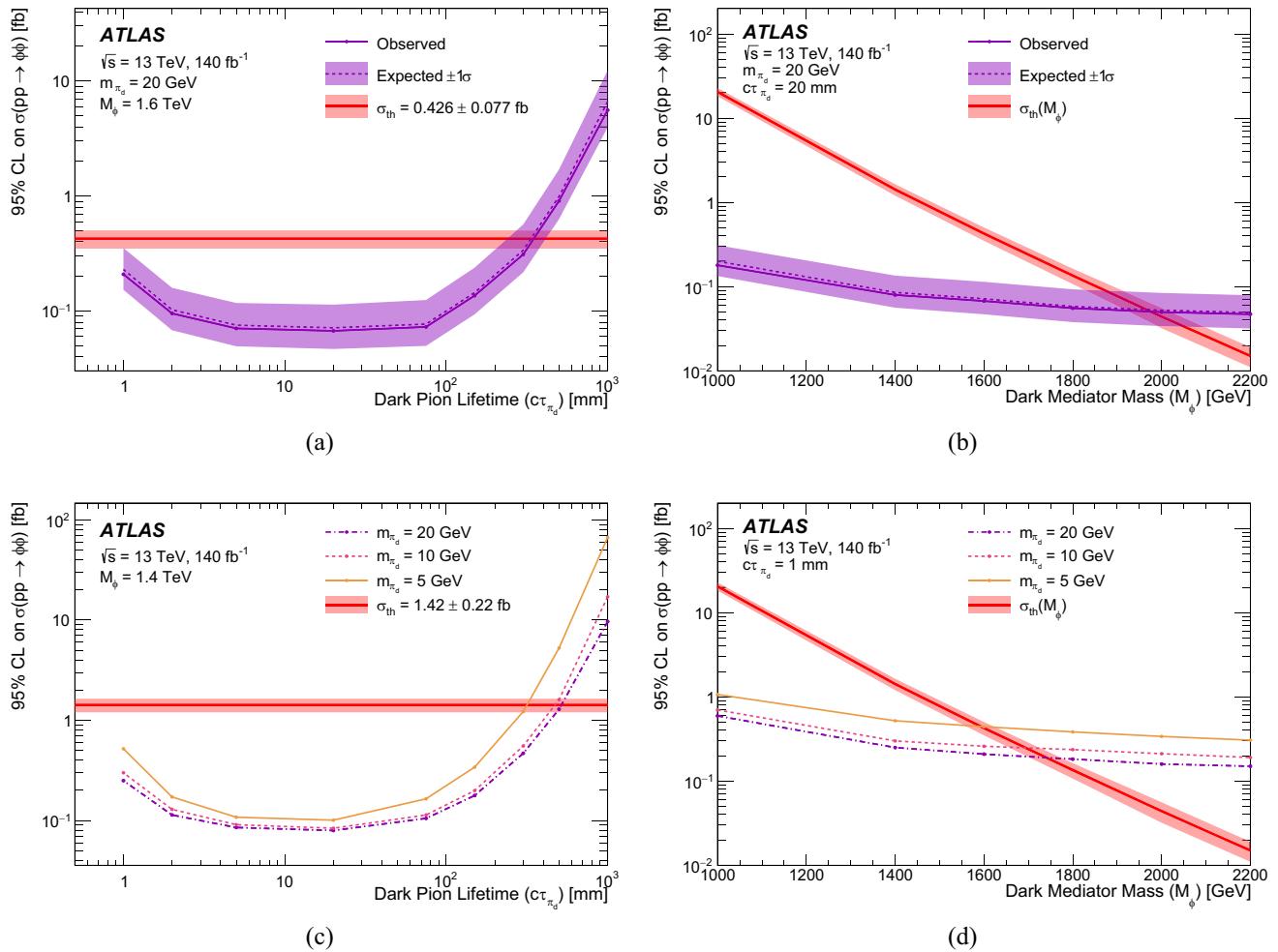
Fig. 6 95% CL upper limits as a function of (left) c\tau_{\pi_d} and (right) M_\phi . The upper plots show the expected and observed limits on \sigma(pp \rightarrow \phi^\dagger\phi) for m_{\pi_d} = 20 GeV: (a) using M_\phi = 1.6 TeV and (b) using c\tau_{\pi_d} = 20 mm. The lower plots show a comparison of the observed
