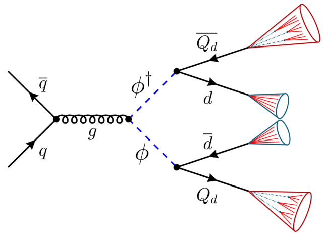
Fig. 1 Feynman diagram of the pair-production of dark scalar mediators, \phi , via quark–antiquark annihilation. The resulting four jets are shown as cones for illustrative purposes. Dashed lines within the cones represent the trajectories of dark pions, solid lines within the cones represent the trajectories of SM particles
