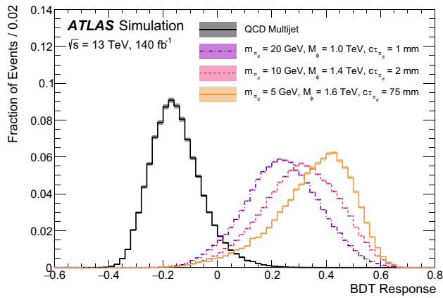
Fig. 2 Normalized event-level BDT response distribution for the QCD multijet background, with three selected signal samples for comparison
