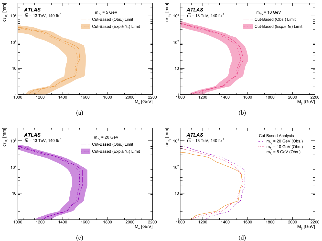
Fig. 11 95% CL exclusion contours as a function of M_\phi and c\tau_{\pi_d} for the Cut-Based analysis. The expected and observed limits on \sigma(pp \rightarrow \phi^\dagger \phi) are shown for (a) m_{\pi_d} = 5 GeV, (b) m_{\pi_d} = 10 GeV, and (c) m_{\pi_d} = 20 GeV. A comparison of the observed limits is given in (d) for each of the three dark pion masses
