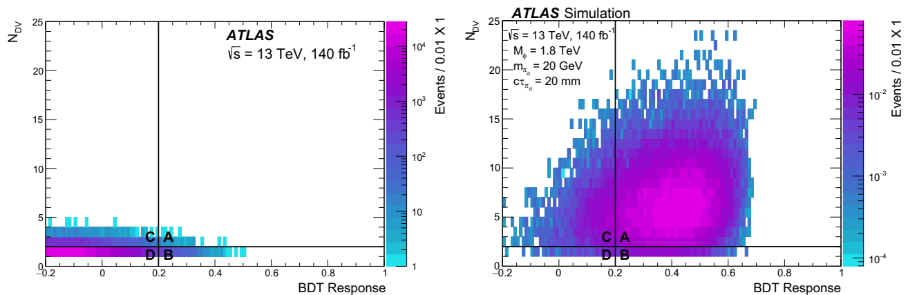
Fig. 3 Distributions of events in the ABCD plane for (left) Run 2 data and (right) an example signal model with parameters: m_{\pi_d} = 20 GeV, M_\phi = 1.8 TeV, and c\tau_{\pi_d} = 20 mm. The signal events are scaled to the
