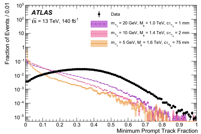
Fig. 9 Normalized minPTF distribution in data, with three selected signal samples for comparison
