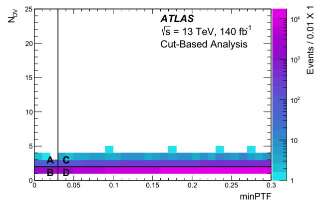
Fig. 10 Distribution of data events in the ABCD plane defined for the Cut-Based analysis, using the minimum prompt track fraction (minPTF) of the four highest p_T jets on the x-axis, and the displaced vertex multiplicity on the y-axis. The cuts used to define the four regions are at minPTF = 0.03 and N_{DV} = 2 . The four regions are labeled accordingly
