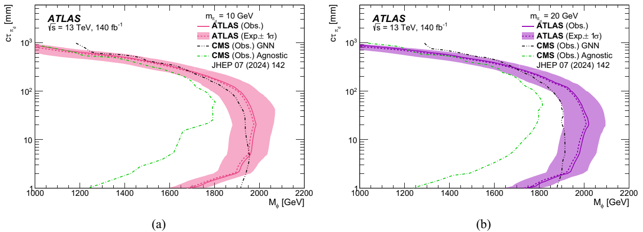
Fig. 8 Comparison of the 95% CL exclusion contours between ATLAS and CMS [28] for (a) models with m_{\pi_d} = 10 GeV and (b) models with m_{\pi_d} = 20 GeV. The expected and observed limits are shown for ATLAS, while only the observed limits in both the model agnostic and
