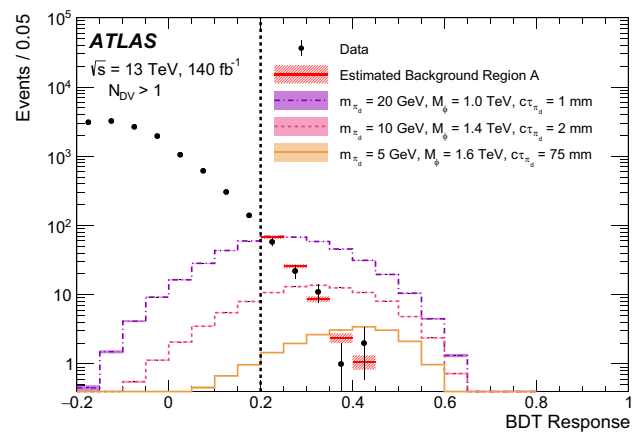
Fig. 5 Comparison of the data with N_{DV} > 1 and the estimated background in the SR using the modified ABCD method. The division between the SR and CR is shown by the vertical dashed line. In the final fit, the bins with R > 0.4 are combined into a single bin. Three selected signal samples are included for comparison
