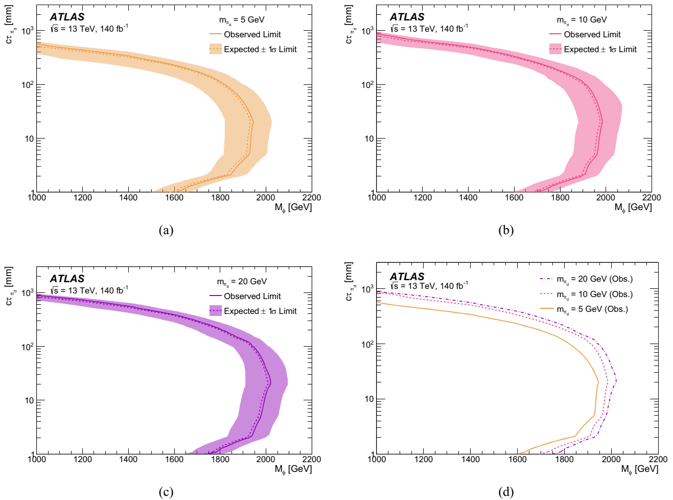
Fig. 7 95% CL exclusion contours as a function of M_\phi and c\tau_{\pi_d} . The expected and observed limits on \sigma(pp \rightarrow \phi^\dagger\phi) are shown for (a) m_{\pi_d} = 5 GeV, (b) m_{\pi_d} = 10 GeV, and (c) m_{\pi_d} = 20 GeV. A comparison of the observed limits is given in (d) for each of the three dark pion masses
