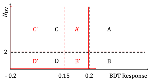
Fig. 4 Schematic diagram of the Shifted-ABCD VR constructed in CRs C and D. The four new regions are shown in red, and labeled A', B', C', and D'. The actual ABCD plane regions are shown in black for comparison
