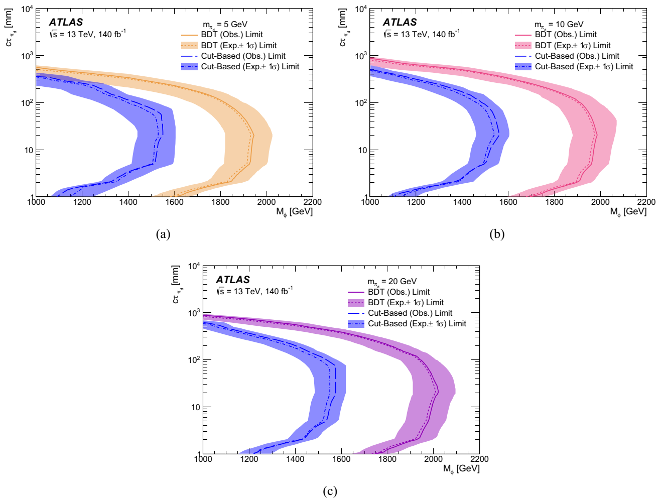
Fig. 12 Comparison of observed and expected 95% CL limits of the Cut-Based analysis against the corresponding BDT-based analysis. Limits on \sigma(pp \rightarrow \phi^+\phi) are shown as a function of M_\phi and c\tau_{\pi_d} for (a) m_{\pi_d} = 5 GeV, (b) m_{\pi_d} = 10 GeV, and (c) m_{\pi_d} = 20 GeV
