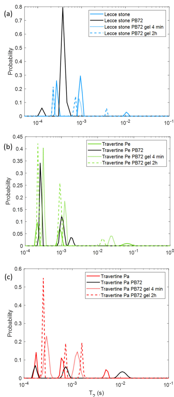
Figure 5. Transversal relaxation time ( T_2 ) distribution for (a) Lecce stone, (b) Travertine Pe, and (c) Travertine Pa before the treatment (solid lines), after PB72 application (black solid lines), and after the PVA-borax gel treatment with application times of 4 min (dotted lines) and 2 h (dashed lines).
