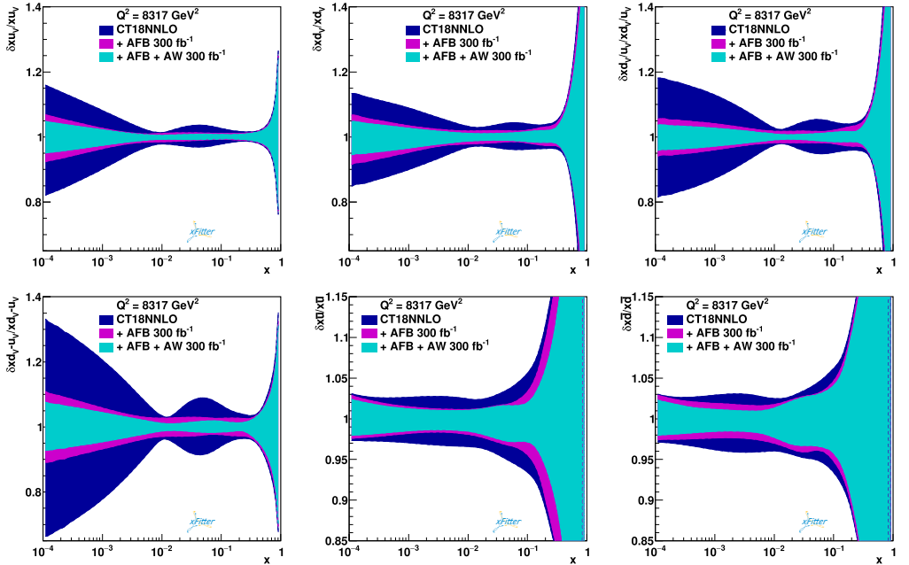
Fig. 6. Original CT18NNLO [34] (blue) and profiled distributions using either A_{FB} (pink) or both A_{FB} and A_W (cyan) pseudodata corresponding to integrated luminosity of 300 \text{ fb}^{-1} . Results are shown for valence-quark and sea-quark distributions at Q^2 = M_Z^2 = 8317 \text{ GeV}^2 .
