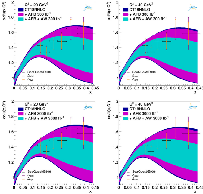
Fig. 8. Profiled error bands with A_{FB} and A_W asymmetries for the \bar{d}/u ratio of PDFs corresponding to 300 (top) and 3000 (bottom) \text{fb}^{-1} at the energy scales Q^2 = 20 \text{ GeV}^2 (left) and Q^2 = 40 \text{ GeV}^2 (right). The SeaQuest/E906 [45] results are superimposed for comparison.
