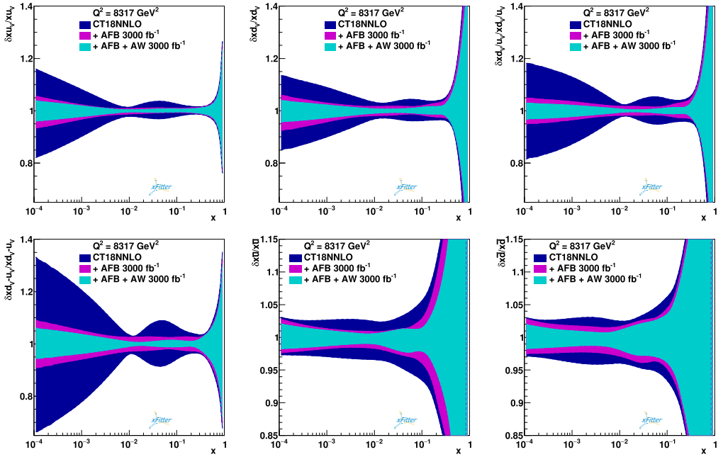
Fig. 7. Same as in Fig. 6 but for integrated luminosity of 3000 fb -1 .
