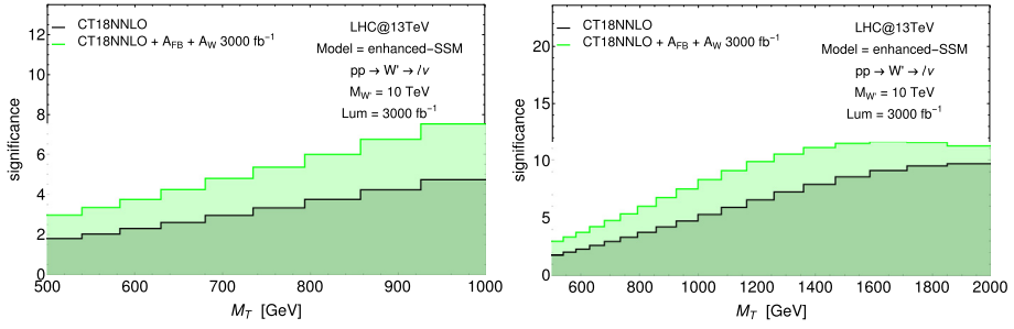
Fig. 17. Significance of the enhanced SSM W' signal with and integrated luminosity of 3000 \text{ fb}^{-1} , including the PDF error from original CT18NNLO PDF set (black) and after the profiling (green) with A_{FB} and A_W pseudodata with the same integrated luminosity accuracy. Efficiencies of both lepton channels are included.
