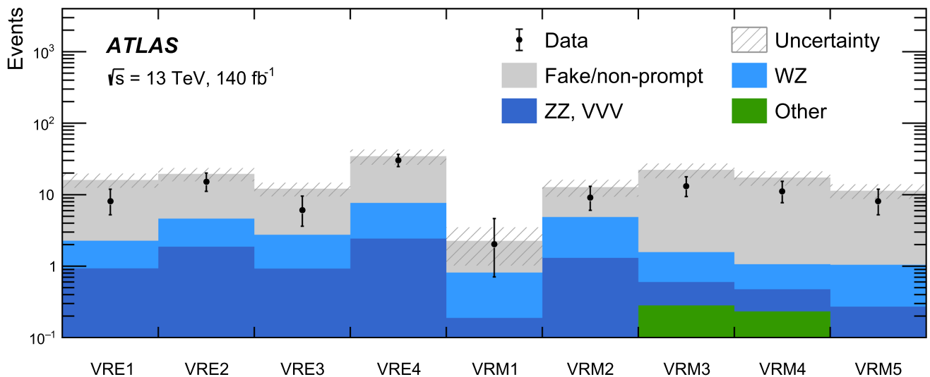
Fig. 3 Comparison between the data and estimated background in the validation regions. The hatched band represents the total uncertainty in the estimated background
