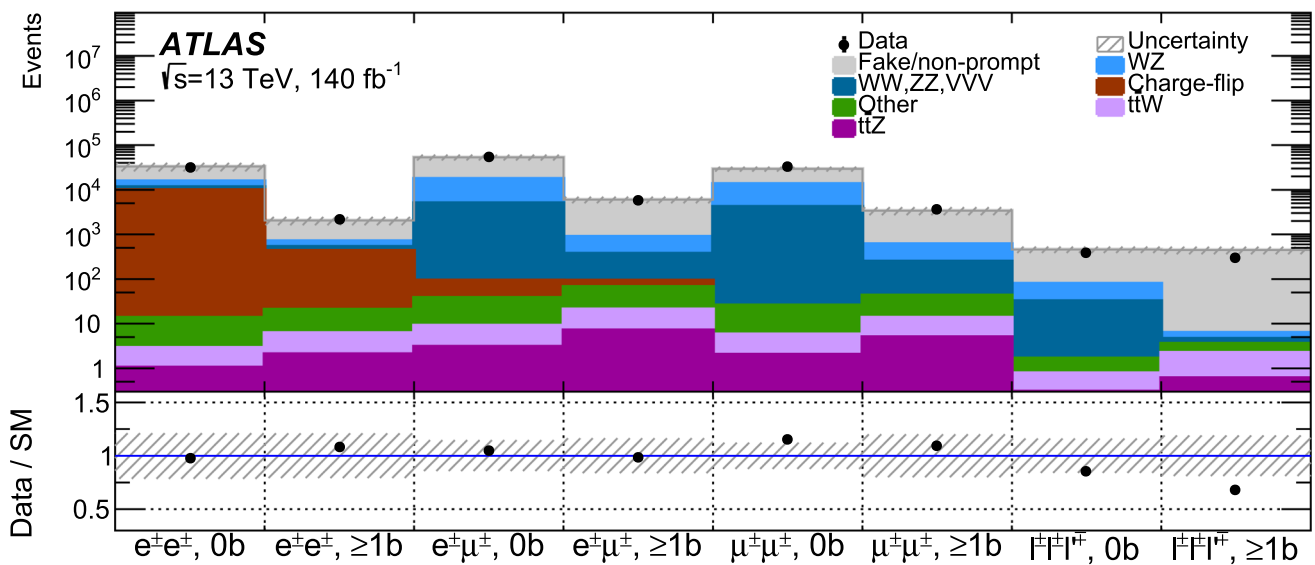
Fig. 2 Comparison between the data and estimated background at pre-selection level. Events entering the SRs defined in Sect. 5 are vetoed. The events are classified in terms of the number of leptons and their flavours, as well as the number of b -jets. The \ell^\pm\ell^\pm bins have a \geq 2 signal leptons selection, with no requirement on the number of base-
