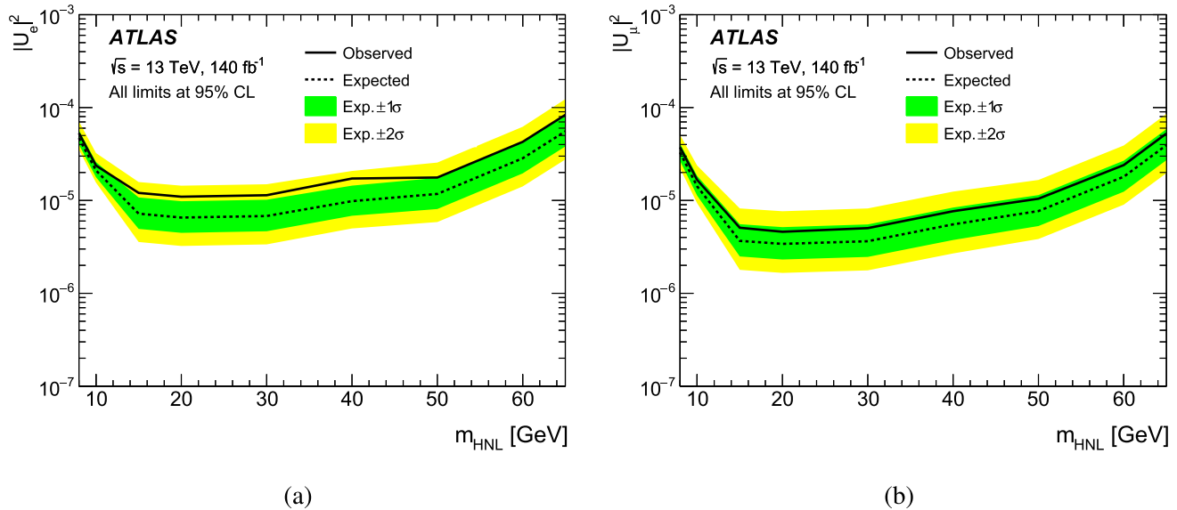
Fig. 4 Observed 95% confidence level (CL) exclusion limits for the (a) |U_e|^2 and (b) |U_\mu|^2 mixing parameters versus the HNL mass. The expected (dashed line) exclusion limits are also shown. The 1\sigma and 2\sigma
