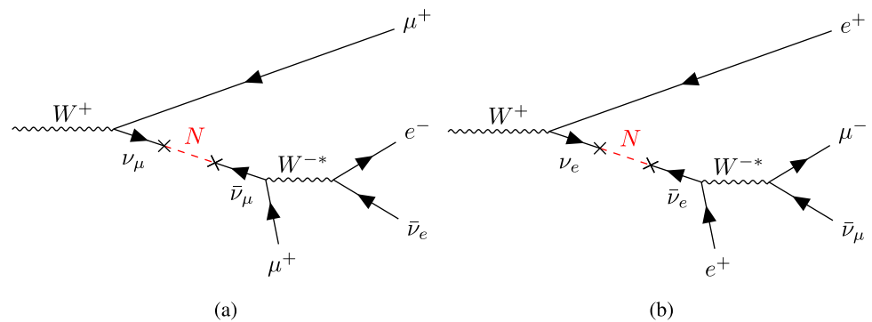
Fig. 1 Feynman diagrams for heavy neutral lepton ( N ) production and decay in the channels originating from: (a) HNL– \nu_\mu mixing and \mu^+e^-\bar{\nu}_e decay of the heavy lepton, and (b) HNL– \nu_e mixing and e^+\mu^-\bar{\nu}_\mu decay of the heavy lepton. Only lepton-number-violating processes are considered
