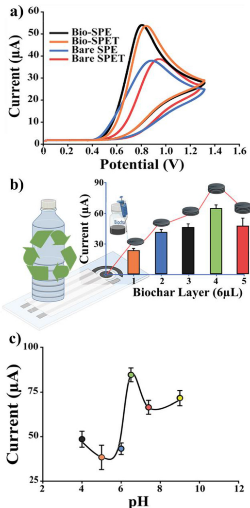
Fig. 4 Optimization of nitrite oxidation using Bio-PET_SPE: (a) voltammograms obtained analysing a constant concentration of NO 2 - (100 μM) using SPEs, PET_SPE, Bio-SPE and Bio-PET_SPE; (b) SWV current as a function of the number of Biochar layers deposited at constant nitrite concentration; (c) currents as a function of pH.
