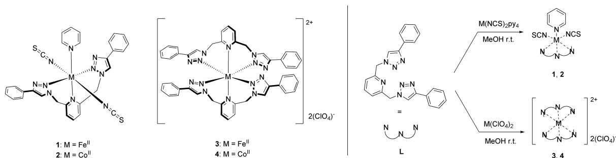
Figure 1. (Left) Chemical structures of the Fe II and Co II complexes investigated as CO 2 reduction CAT in this work. (Right) Synthetic pathways of the heteroleptic ( 1 and 2 ) and homoleptic ( 3 and 4 ) complexes in methanol at room temperature.
