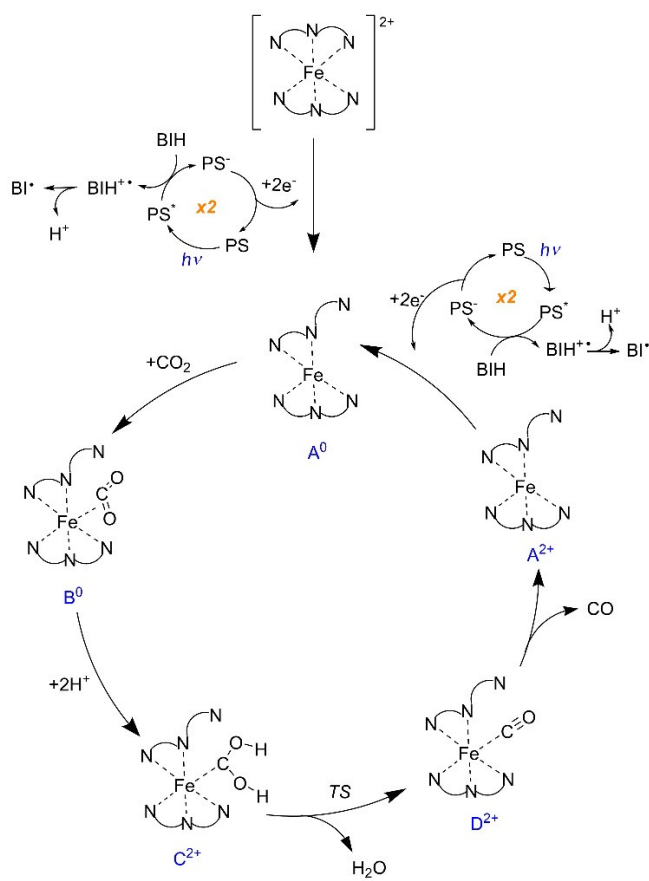
Scheme 2. Proposed mechanism for the photocatalytic CO 2 reduction with 3.
