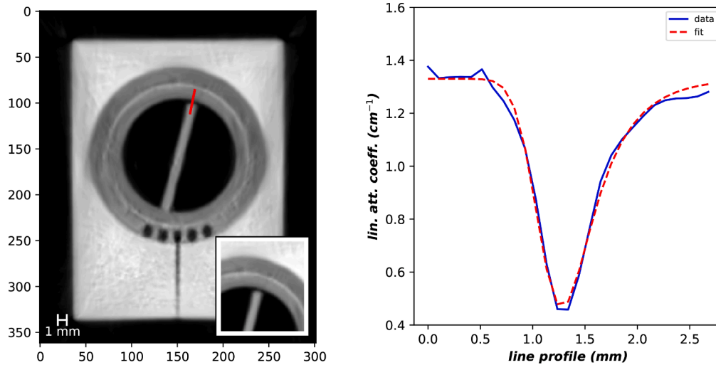
Fig. 15. Example of the gap between the swirl tape with the pipe's internal surface for the CCFE9 mock-up.
