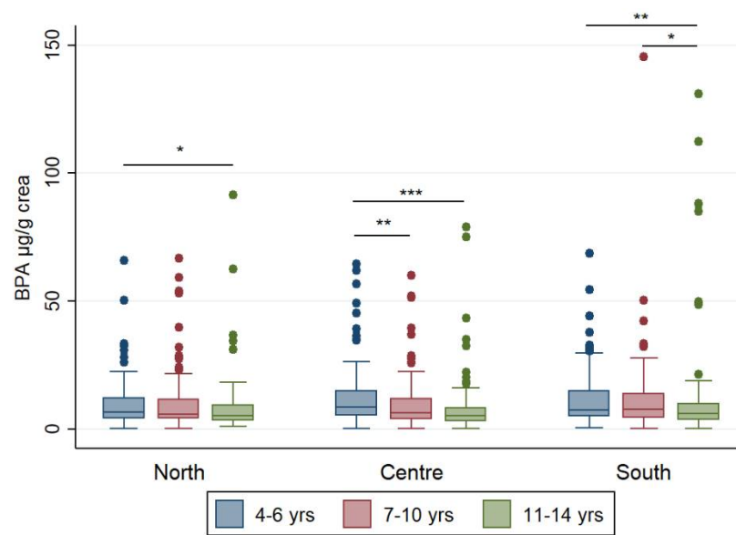
Figure 2. Box plots for BPA levels in urine samples of Italian children stratified by macro-area and age classes and normalized to urine creatinine content ( \mu\text{g/g} crea). Outliers above 150 \mu\text{g/g} crea were excluded from the graph to improve box plot visibility. Asterisks indicate the level of significance: * p < 0.05 , ** p < 0.01 , *** p < 0.001 .
