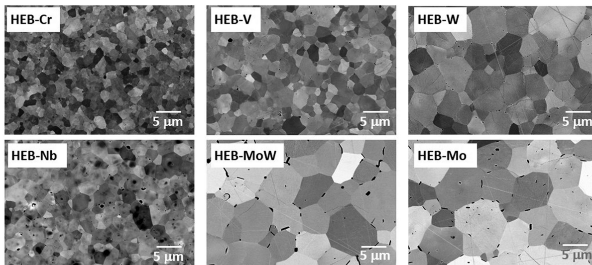
FIGURE 2 BSE-FESEM micrographs from a polished surface, taken at the same magnification. The nature of the black spots in HEB- x ( x = \text{Nb} , \text{MoW} , or \text{Mo} ) is described in the main text. Residual scratches due to polishing are still visible in HEB- x ( x = \text{V} , \text{W} , \text{MoW} , and \text{Mo} )
