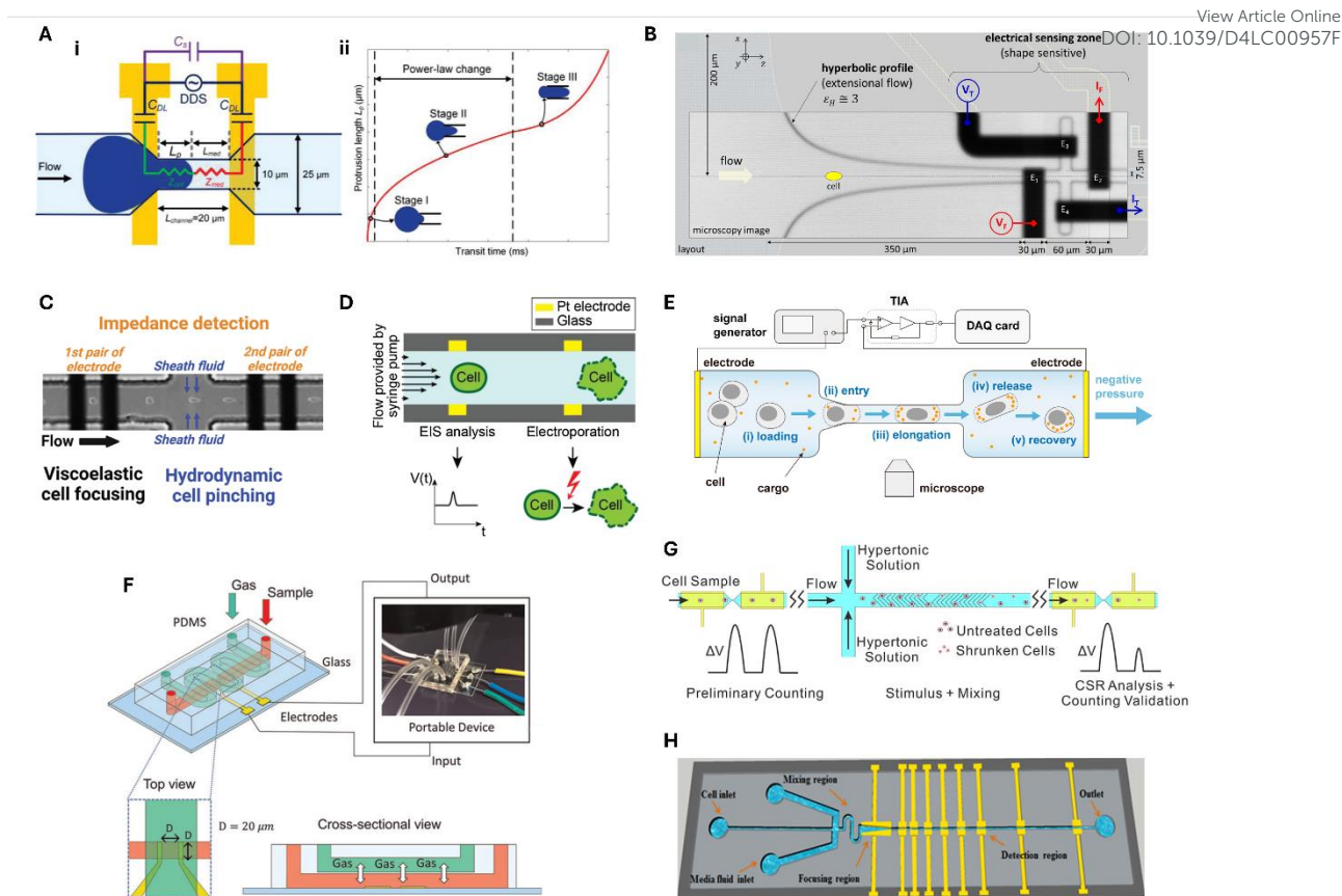
Fig. 4 Examples of microfluidic systems integrating MIC-sensing with on-chip sample stimulation. (A) Single-cell intrinsic mechanical characterization by ref. 78 : i) equivalent impedance-deformability mapping model and ii) protrusion length time-course. (B) Layout of the system developed in ref. 71 consisting of a hyperbolic microchannel, inducing cell deformation by extensional flow, equipped with shape-sensitive MIC electrodes. (C) Brightfield image illustrating hydrodynamic cell deformation by sheath fluid at the channel cross junction, by ref. 81 . (D) Cross-sectional schematic of the chip from ref. 85 : a pair of electrodes for electroperoration upon passage of a cell, and a separate set of two facing electrodes for EIS measurements. (E) Schematic of the microfluidic system for single-cell electroperoration and impedance assessment from ref. 86 (TIA, trans-impedance amplifier, DAQ, data acquisition). (F) Schematics and picture of the portable MIC system with oxygen control developed in ref. 88 . (G) Design principle of the microfluidic hypertonic stimulus-based impedance flow cytometry chip from ref. 89 . (H) Schematic of the microfluidic platform structure for membrane permeability measurement by ref. 90 . Images were adapted with permission from (A) ref. 78 , copyright 2022 Wiley-VCH GmbH, (B) ref. 71 , copyright 2022 IEEE, (C) ref. 81 , copyright 2022 Wiley-VCH GmbH, (D) ref. 85 , copyright 2014 Elsevier B.V., (E) ref. 86 , copyright 2020 The Authors, (F) ref. 88 , copyright 2021 Wiley Periodicals LLC, (G) ref. 89 , copyright 2019 Elsevier B.V., (H) ref. 90 , copyright 2021 Elsevier B.V.
