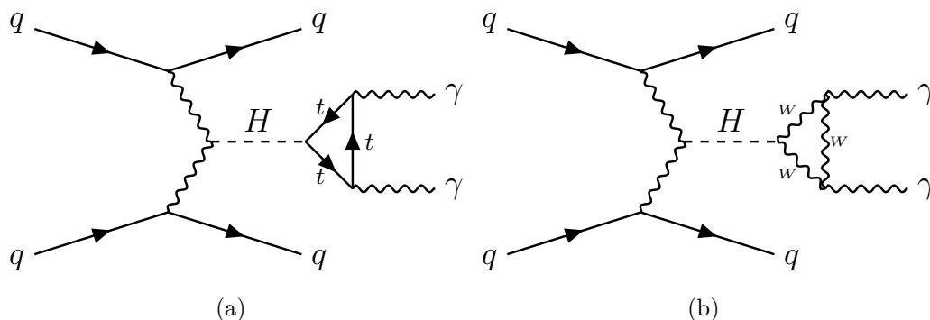
Figure 1. Representative lowest-order Feynman diagrams of vector-boson fusion production of a Higgs boson and subsequent decay into two photons H \rightarrow \gamma\gamma via (a) a top-quark loop and (b) a W -boson loop.
