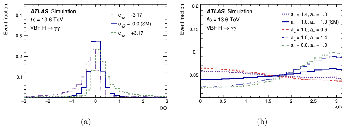
Figure 2. Distributions of (a) the \mathcal{OO} observable shown for various configurations of the Wilson coefficient c_{H\tilde{W}} , and (b) the \Delta\Phi_{jj} observable for various configurations of the a_L and a_T parameters. These comparisons are performed in VBF events at the reconstruction level using the predictions of the MADGRAPH5_AMC@NLO + PYTHIA 8 [41, 43] generators.
