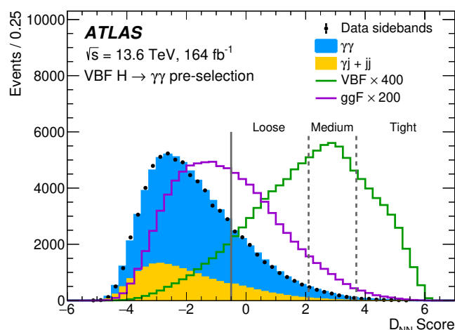
Figure 3. Comparison of the NN response score ( D_{\text{NN}} ) distributions for the VBF signal, the ggF background, and the non-resonant background, overlaid with sideband data. The non-resonant background includes simulated \gamma\gamma continuum events as well as \gamma + j and jj processes where one or more jets are misidentified as photons; the latter are estimated from control regions in data as detailed in section 7. The VBF signal and ggF background are scaled by factors of 400 and 200 relative to their SM expectations, respectively. Vertical dashed lines indicate the thresholds used to define the signal categories, while events with a D_{\text{NN}} score below the lowest threshold (solid line) are excluded from the analysis.
