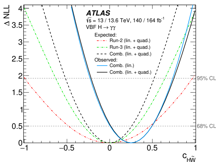
Figure 10. Expected and observed likelihood curve as a function of the Wilson coefficient c_{H\tilde{W}} . The results are shown for the individual Run-2 and Run-3 datasets, as well as for the combined fit of both datasets. Scans are performed using both the full linear+quadratic and linear-only parameterisations. The dashed horizontal lines indicate the \Delta\text{NLL} values corresponding to the 68% and 95% CL intervals. Results are obtained assuming a new physics scale of \Lambda = 1 TeV.
