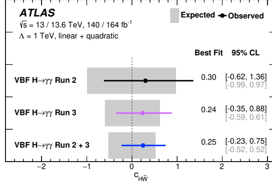
Figure 7. The expected and observed measurements of the Wilson coefficient c_{H\tilde{W}} in the VBF H \rightarrow \gamma\gamma channel. Results are shown for integrated luminosities of 140 \text{ fb}^{-1} at \sqrt{s} = 13 \text{ TeV} [21] and 164 \text{ fb}^{-1} at \sqrt{s} = 13.6 \text{ TeV} , and for the statistical combination of both data samples (as presented in section 9.2). The dots and 95% CL bars show the best-fit values with statistical and systematic uncertainties, and the grey bands centred at zero show the expected 95% CL intervals. The best fit values and 95% CL observed (expected) limits are also explicitly stated on the right-hand side of the plot in black (grey). Results are obtained assuming a new physics scale of \Lambda = 1 \text{ TeV} .
