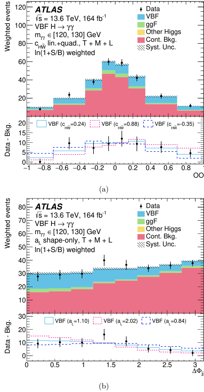
Figure 4. Post-fit distributions of (a) the optimal observable and (b) \Delta\Phi_{jj} for events in the combined tight (T), medium (M), and loose (L) analysis regions within the invariant diphoton mass window m_{\gamma\gamma} \in [120, 130] \text{ GeV} . The signal and background yields are fixed to the best-fit values from the c_{H\tilde{W}} and a_L interpretations. Contributions from the three regions are summed, weighted by \ln(1+S/B) , where S and B are the best-fit signal and background yields, respectively. The overflow and underflow are included in the outermost bins. The uncertainty band includes all systematic uncertainties. The lower panels show the background-subtracted data compared with the best-fit VBF prediction and two BSM scenarios corresponding to the two POI values excluded at exactly 95% CL by fits using only shape information.
