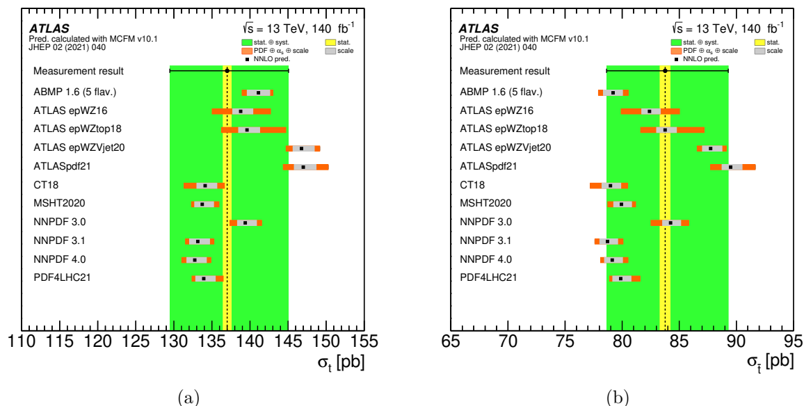
Figure 13. Comparison of NNLO predictions based on several different PDF sets with the measured values (dots) of (a) \sigma(tq) and (b) \sigma(t\bar{q}) . The yellow band represents the statistical uncertainty and the green band the total uncertainty. The uncertainties in the theoretical predictions include PDF, scale and \alpha_s uncertainties.
