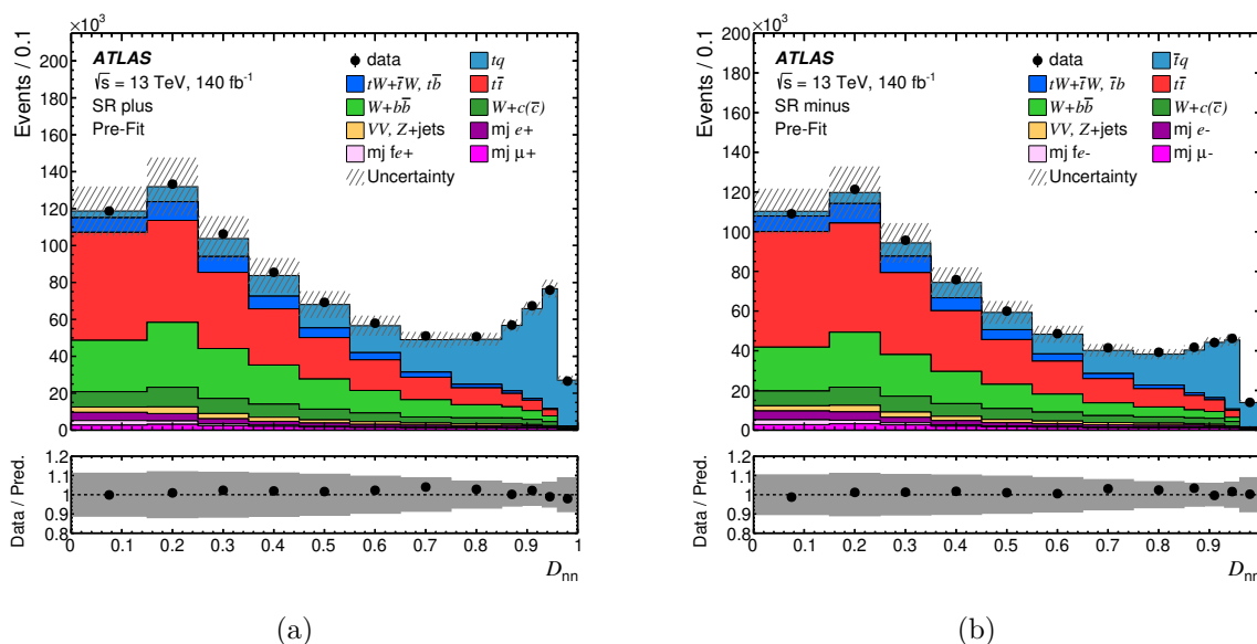
Figure 6. Pre-fit distributions of the D_{nn} in (a) SR plus and (b) SR minus. The observed distributions (dots) are compared with the expected distributions (histograms) from simulated events. In these distributions, the signal contribution is shown stacked on top of contributions from all considered background processes. All uncertainties considered in the analysis are included in the hatched uncertainty band. The lower panel shows the ratio of data and the prediction; in this panel, the uncertainty is displayed as a grey band.
