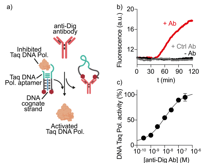
Figure 4. a) Antibody-protein communication to control Taq DNA polymerase activity. b) Taq DNA polymerase activation followed through kinetic traces in presence of anti-Dig antibodies (300 nM). No activation is observed in absence of anti-Dig antibodies and at high concentrations (300 nM) of a control antibody (grey curve). c) Anti-Dig antibodies concentration-dependent regulation of Taq polymerase activity. For experimental conditions see SI.
