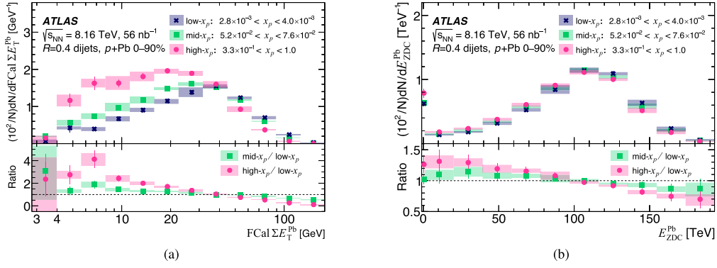
Fig. 2. (a) FCal \Sigma E_T^{\text{Pb}} and (b) E_{\text{ZDC}}^{\text{Pb}} distributions plotted for low-, middle-, and high- x_p selections. These distributions are normalized to display the change of shape with x_p . The bottom panel displays the ratio of the middle- and high- x_p selection over the low- x_p selection. In sub-figure (b) the energy below the ZDC detection threshold (e.g., formally assigned as zero by ZDC reconstruction) is reported in a dedicated bin. Please note that results in each bin are divided by the bin width. This is relevant in sub-figure (b) comparing the zero energy bin to the rest of the distribution. Vertical error bars represent the statistical uncertainty, and the shaded areas represent the systematic uncertainty. The width of the shaded area indicates the bin width.
