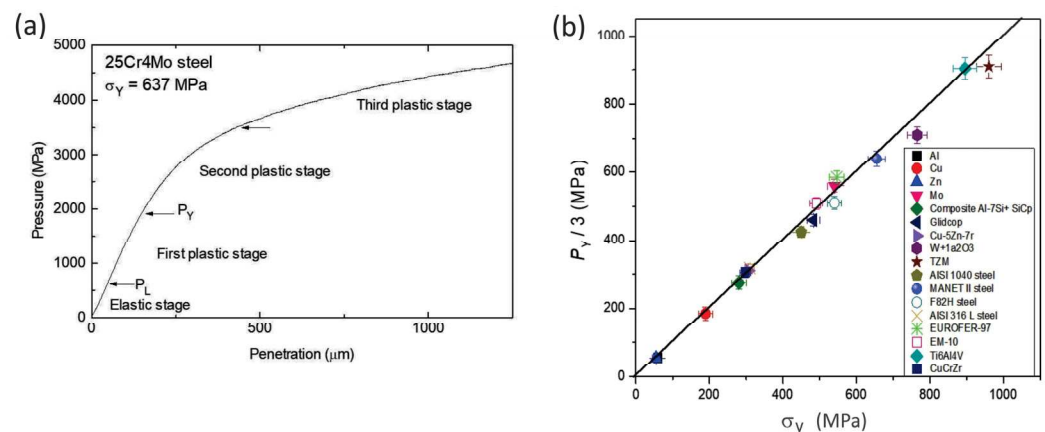
Figure 12. Results of the FIMEC test for different materials: (a) Typical indentation curve; (b) Assessment of the relationship \sigma_Y = P_Y/3 (Reproduced from [39]).
