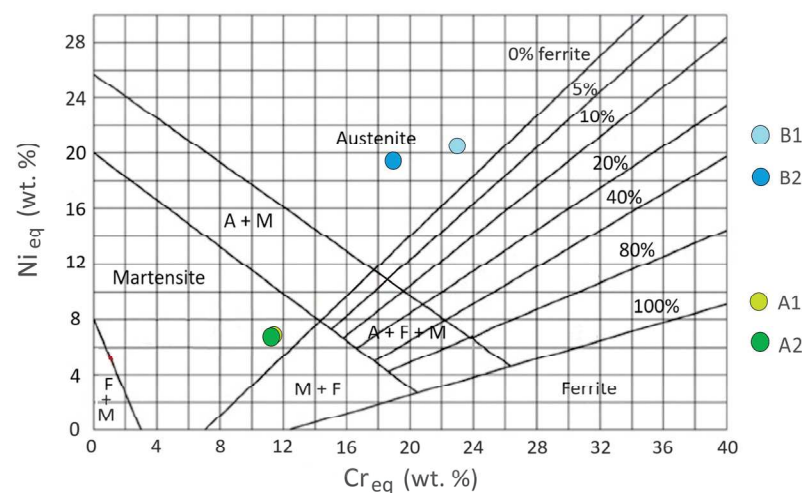
Figure 17. Schaeffler diagram with indication of the points representative of the FZ composition for the specimens A (points A1 and A2 as in Figure 11) and B (points B1 and B2 as in Figure 11).
