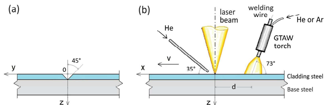
Figure 4. Welding setup: (a) Preparation of the two clad steel plates in the cross-section plane; (b) Laser-leading configuration.
