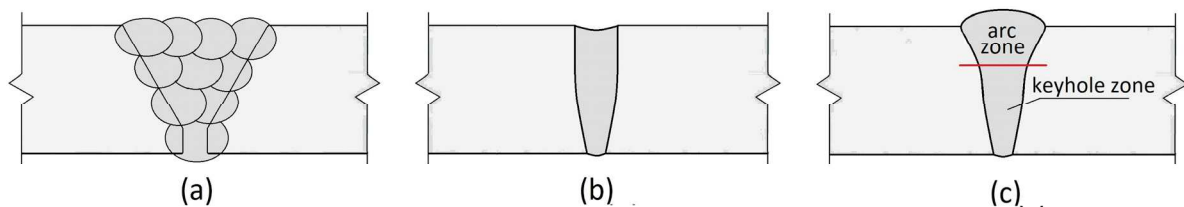
Figure 1. Sketches of the sections obtained respectively by: (a) Multi-pass arc welding; (b) Single pass of LBW; (c) Single pass of LAHW.
