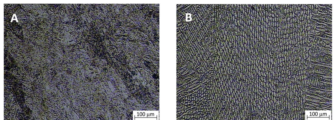
Figure 7. Dendritic microstructures of FZ near the weld centerline of the two specimens.
