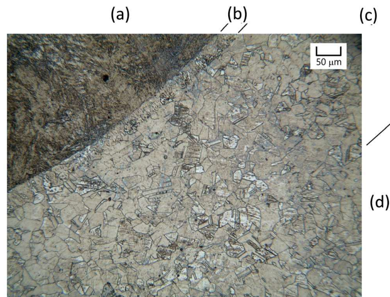
Figure 8. Optical micrograph of the interface weld/austenitic parent metal (specimen A): (a) Dendrites (FZ); (b) Thin layer with small austenitic grains (HAZ); (c) Slightly enlarged grains (HAZ); (d) Austenitic parent metal.
