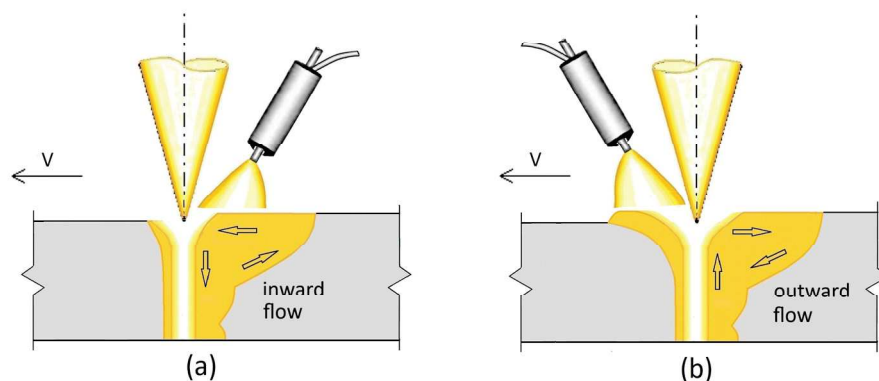
Figure 2. LAHW configurations (vector v represents the welding speed direction): (a) Laser beam leading; (b) Arc leading.
