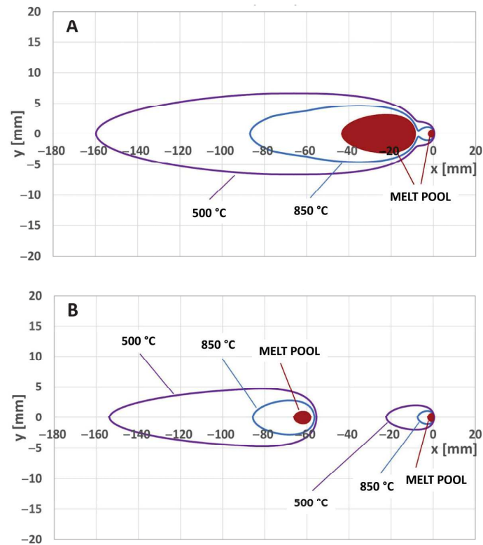
Figure 14. Thermal simulation results for the two procedures: melt pools (filled shapes with contours at T = T_m ) and isotherms at 850 °C and 500 °C in the xy plane, calculated at the interface between the cladding layer and the base metal ( z = 2.5 mm).
