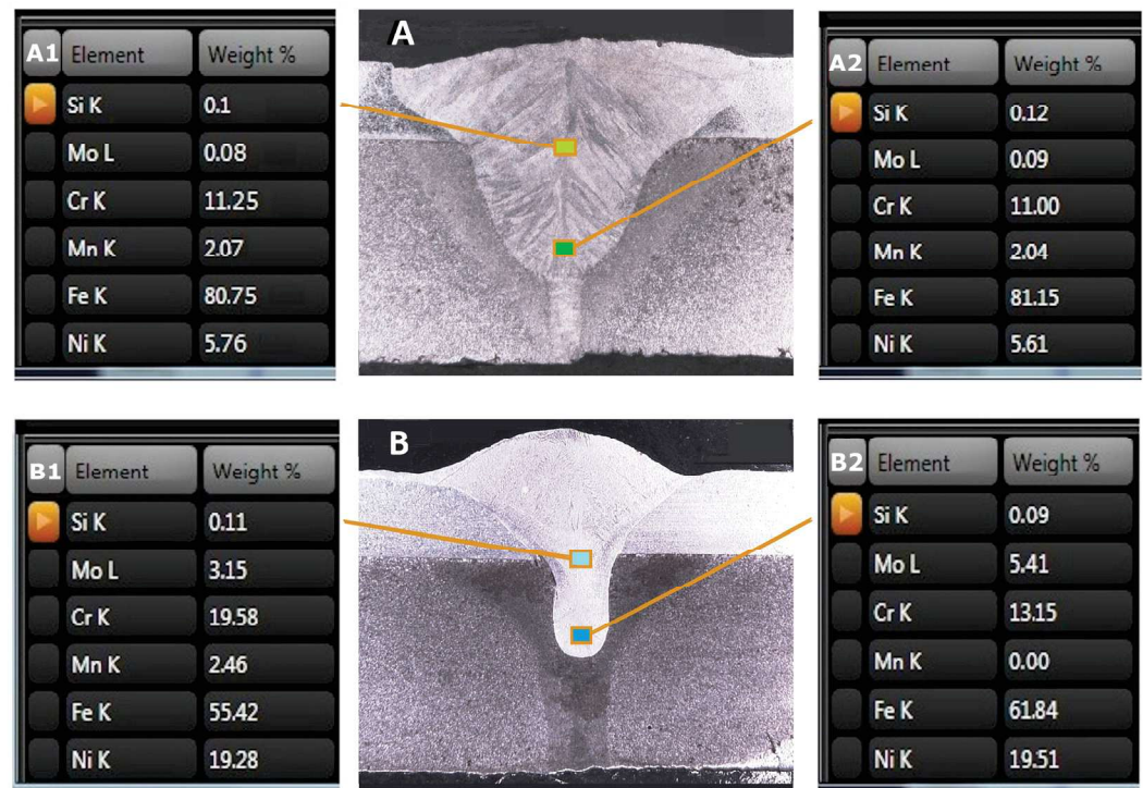
Figure 11. Results of EDS measurements on two representative points in the cross-section for both specimens (A,B).
