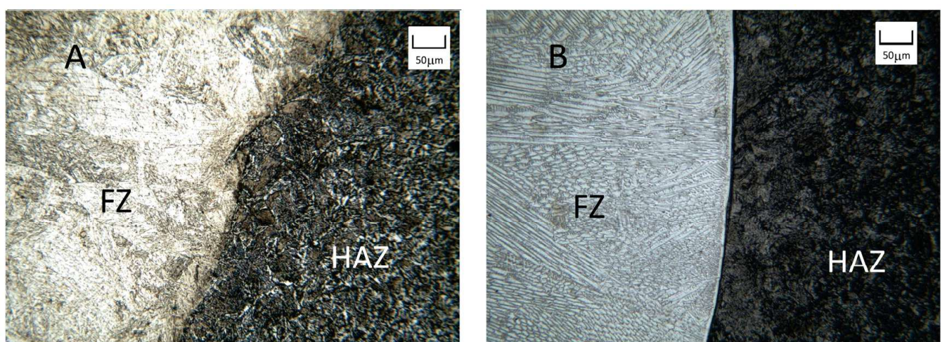
Figure 9. Optical micrographs of the interface FZ/A 515 Gr. 60 base plate for the two specimens.
