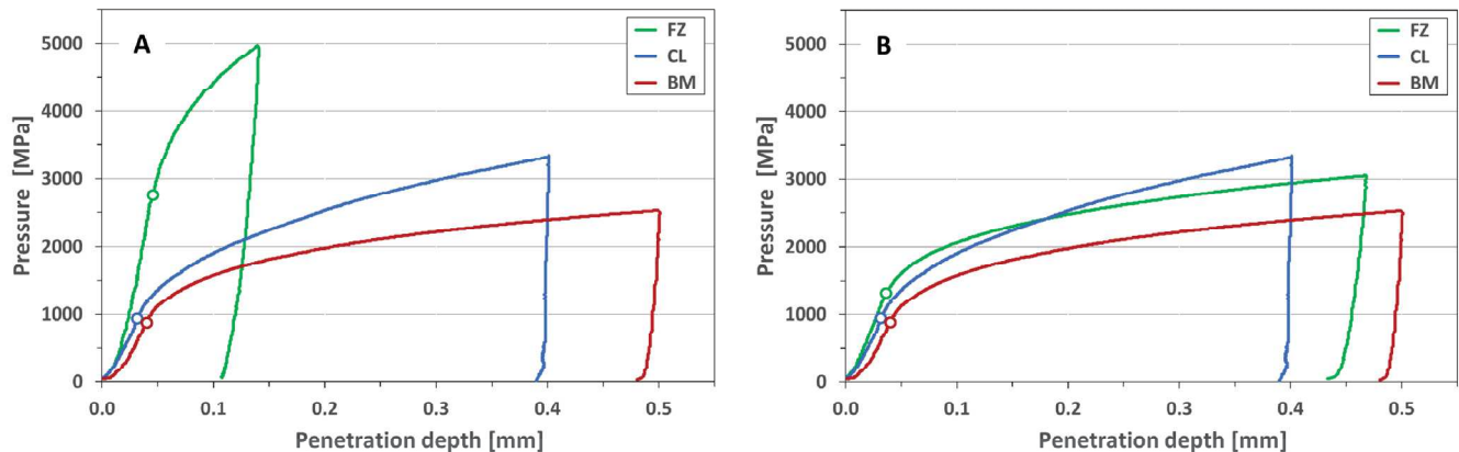
Figure 13. Results of FIMEC test for specimens (A,B).
