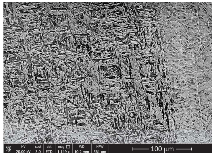
Figure 10. SEM micrograph taken on the FZ centerline of the specimen A.
