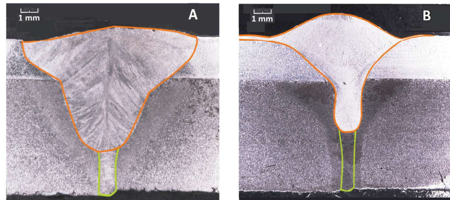
Figure 16. Cross sections of the specimens A and B, with the areas welded by the electric arc (orange) and by the laser beam (green) outlined.
