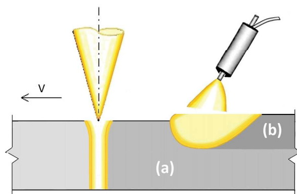
Figure 3. Sketch of the tandem configuration with indication of the welding speed v direction: (a) Deep weldment produced by the keyhole; (b) Shallow weldment due to the electric arc.
