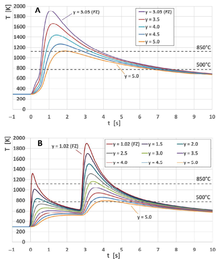
Figure 15. Thermal simulation results for the two procedures: temperature profiles for fixed points located at the interface between the cladding layer and the base metal ( z = 2.5 mm), parameterized according to the y coordinate (distance of the point from the welding line at the interface).
