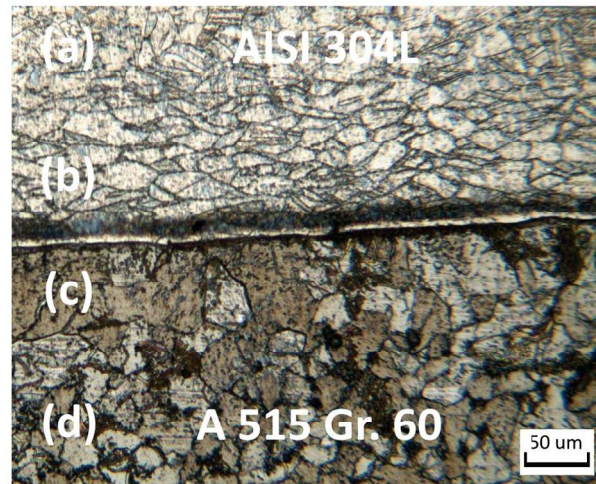
Figure 6. Optical micrograph of the interface between AISI 304 L and ASTM A515 Gr. 60 with indication of the microhardness values: (a) Austenitic cladding layer; (b) Sensitized zone; (c) Decarburized zone; (d) Base carbon steel.
