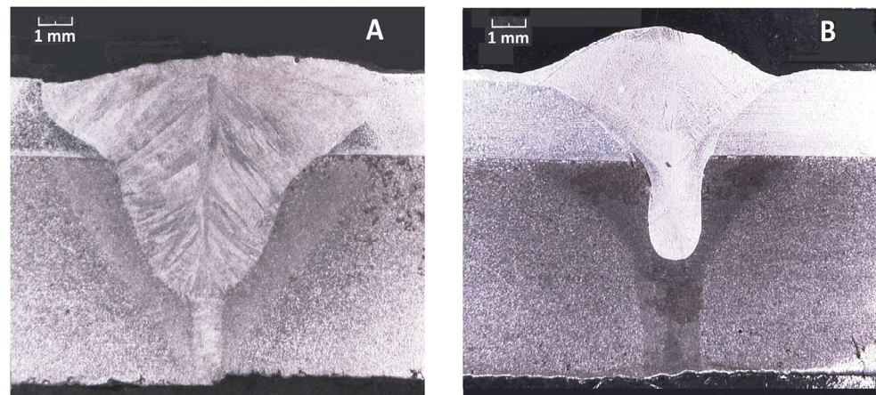
Figure 5. Cross-sections of the welds obtained with the two welding procedures (A,B).
