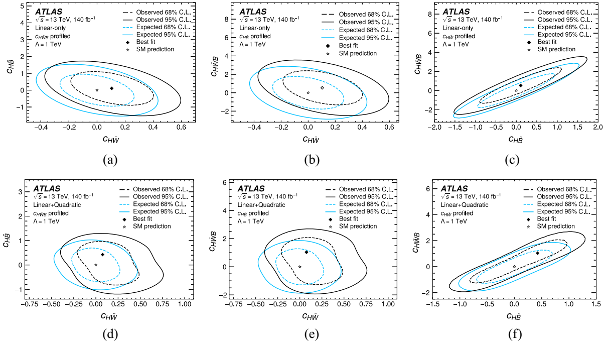
FIG. 3. Observed 68% (dashed line) and 95% (solid line) C.L. two-dimensional contours are shown for all three pairings of the Warsaw basis: (a),(d) c_{H\bar{W}} versus c_{H\bar{B}} , (b),(e) c_{H\bar{W}} versus c_{H\bar{W}B} , and (c),(f) c_{H\bar{B}} versus c_{H\bar{W}B} a simultaneous fit, for (a)–(c) linear-only and (d)–(f) linear plus quadratic terms interpretations. Expected contour lines are also shown. All couplings scale as 1/\Lambda^2 with \Lambda = 1 TeV.
