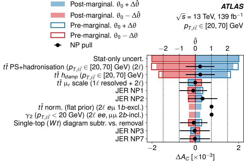
(a) 20 < p_{T,\ell\bar{\ell}} < 70 GeV
