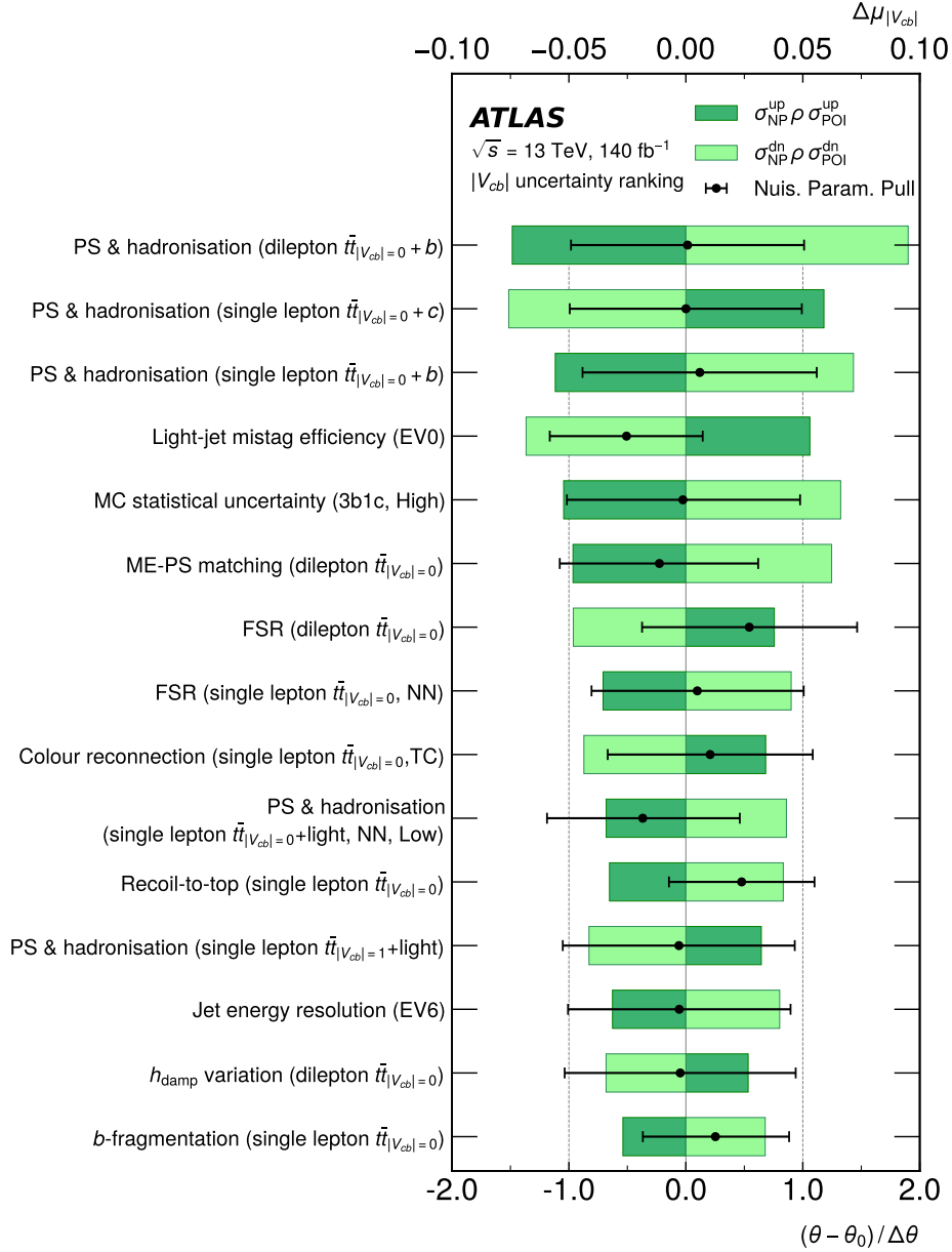
Figure 7. Ranking of the fifteen most significant impacts of individual systematic uncertainties in \mu_{|V_{cb}|} using the covariance method. The dots shows the post-fit value of each nuisance parameter, and the associated band shows the post-fit uncertainty of the parameter. Uncertainties that are decorrelated between samples or regions are labelled with the corresponding sample or region in parentheses. The light-jet mistag efficiency and jet energy resolution uncertainties are split into components; the parentheses indicate the most impactful component.
