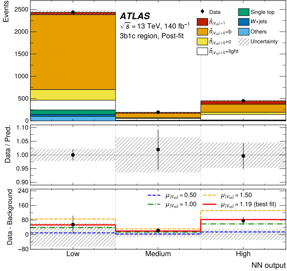
Figure 6. Post-fit distribution of the NN output in the 3b1c region. The upper panel shows the data yield in each bin, and the fitted background and signal MC samples. The middle panel shows the ratio between data and MC. The shaded region marks the total systematic uncertainty, while the error bar on the data symbols represents the statistical uncertainty. The bottom panel shows the data with the background (all samples, excluding t\bar{t}_{|V_{cb}|=1} ) subtracted, with the lines showing the expected number of t\bar{t}_{|V_{cb}|=1} events at different values of \mu_{|V_{cb}|} , together with the best fit value.
