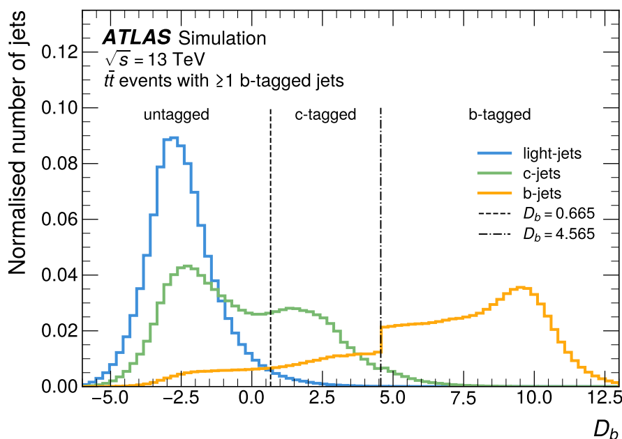
Figure 2. Distribution of the D_b scores for jets from t\bar{t} events after applying the event selection requirements detailed in the text, with the thresholds used to define c - and b -tagged jets shown. For visualisation purposes, the distributions for each flavour are normalised such that the plotted numbers of true light-, c -, and b -jets are equal. Since at least one b -tagged jet is required in the event selection, there is a step in the distribution at the b -tag D_b threshold.
