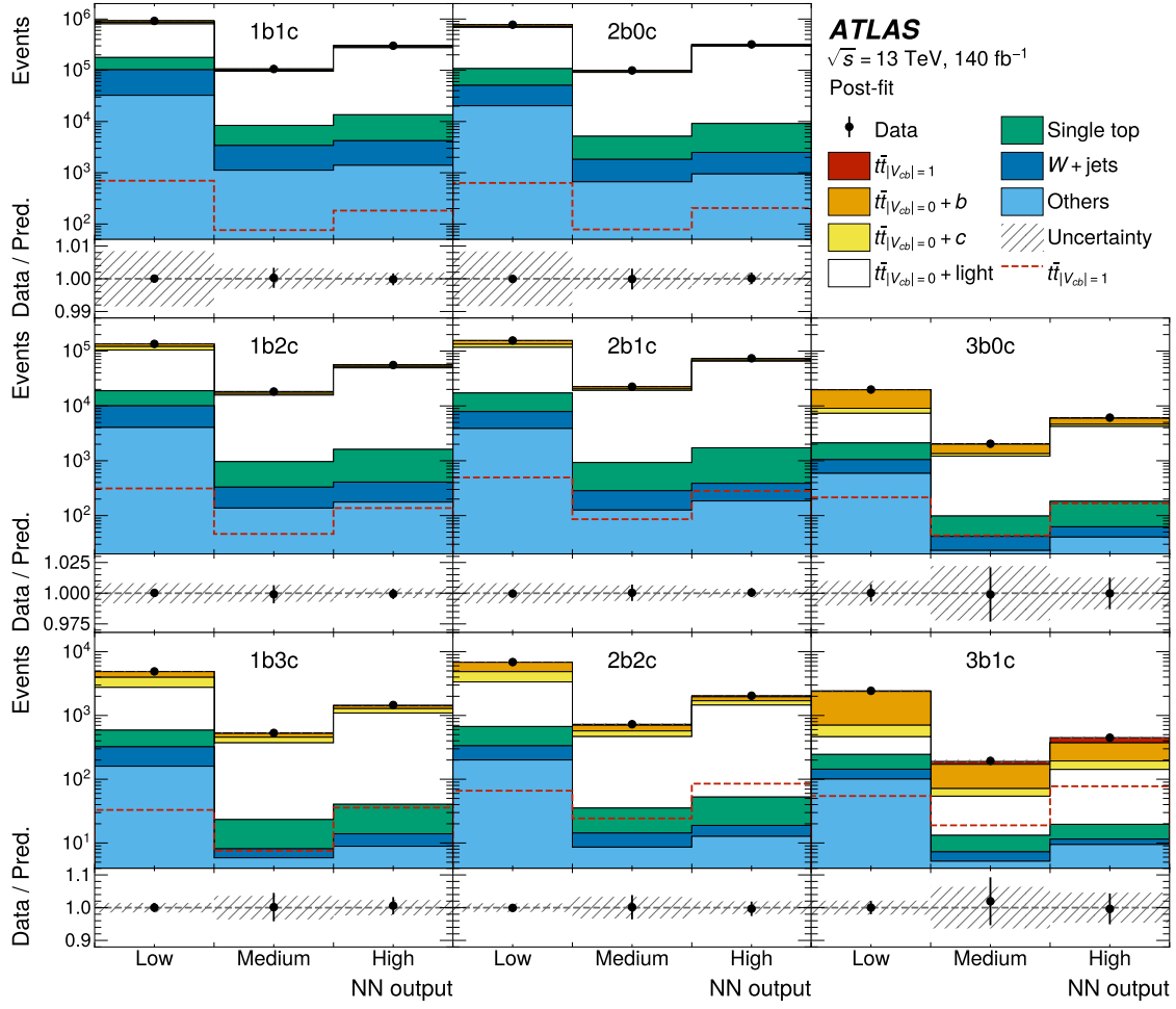
Figure 5. Post-fit distributions of the data and predicted event yields across all bins used in the fit. Each panel in the grid represents a tagging category (1b1c–3b1c), showing the event yields in the three Neural Network (NN) output score bins (Low, Medium, High). The grid is organised such that regions in the same row contain the same total number of heavy-flavour ( b or c ) jets and share the same y -axis scales, while regions in the same column contain the same number of b -jets. The data are shown as closed circles with statistical uncertainties; the prediction is shown as stacked histograms, broken down into the signal |V_{cb}| = 1 and background processes. The signal |V_{cb}| = 1 process is also separately overlaid for visualisation. The hatched bands represent the total systematic uncertainties. The lower panels show the ratios of the data to the predictions.
