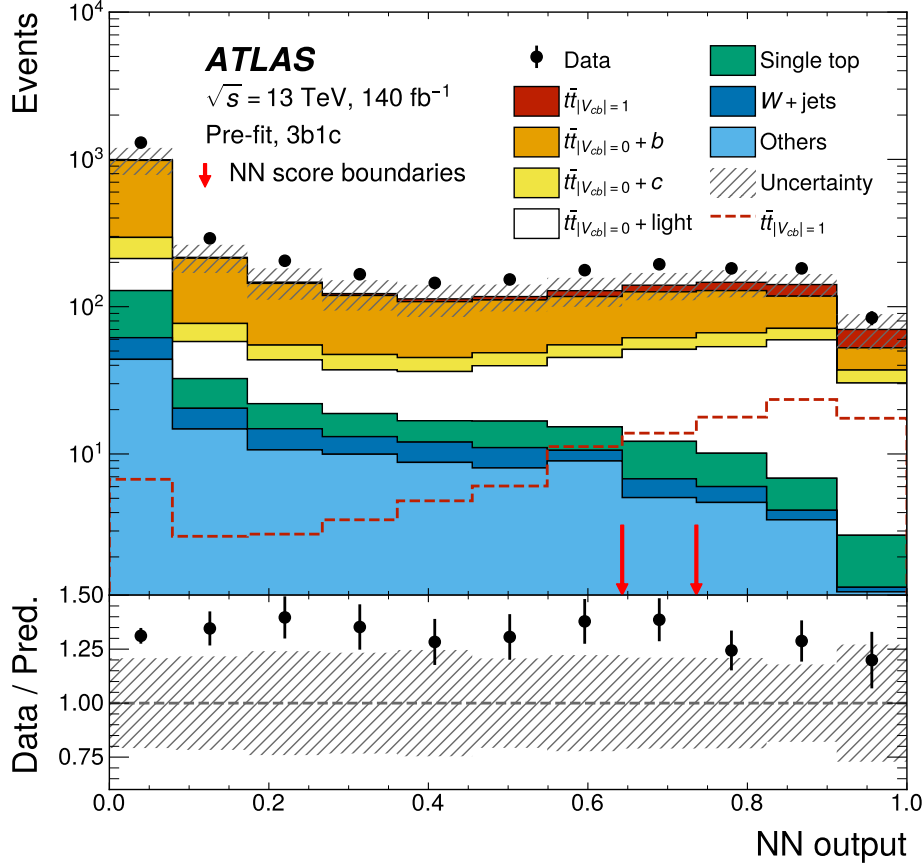
Figure 3. Pre-fit distribution of the Neural Network (NN) output score in the 3b1c tagging category. The data are shown as closed circles with statistical uncertainties; the prediction is shown as stacked histograms, broken down into the signal |V_{cb}| = 1 and background processes. The signal |V_{cb}| = 1 process is also overlaid separately for visualisation. The hatched bands represent the total systematic uncertainties. The lower panels show the ratios of the data to the prediction. The arrows indicate the optimised bin boundaries that are used in the profile-likelihood fit. The “Others” category consists of Z +jets, diboson, t\bar{t} + H/W/Z and multijet events.
