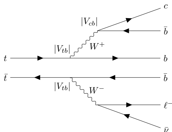
Figure 1. Leading-order Feynman diagram describing the t\bar{t} \rightarrow bW^+ \bar{b}W^- \rightarrow \bar{b}c \bar{b}l^- \bar{\nu} decay. Vertices are labelled with the appropriate CKM matrix elements.
