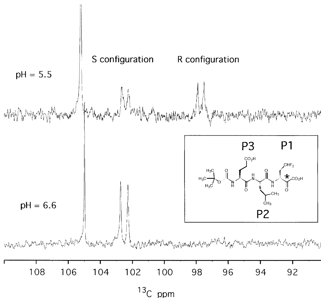
Fig. 3. The inset shows the reversible covalently bound inhibitor \alpha -ketoacid Boc-Glu-Leu-( \gamma -di-fluoro)Abu; the corresponding positions in the substrate-like nomenclature (P1, P2 and P3) are also indicated. The asterisk labels the activated carbonyl moiety, which acts as binding group and becomes the hemiketal chiral carbon upon complex formation. The spectra show regions of the 1D ^{13}\text{C} experiment where the hemiketal carbon of the complex resonates. At pH 6.6 (bottom) only one doublet resonance is visible at 102.6 p.p.m., corresponding to the S configuration; at pH 5.5 (top), two resonances of similar intensity appear at 102.6 and 97.6 p.p.m. for the R and S configurations, respectively. The hemiketal signals are doublets since they are coupled with the \alpha -C, which is also ^{13}\text{C} labelled, while the carboxyl atom is unlabelled. The intense singlet at ~105 p.p.m. represents a buffer resonance.
