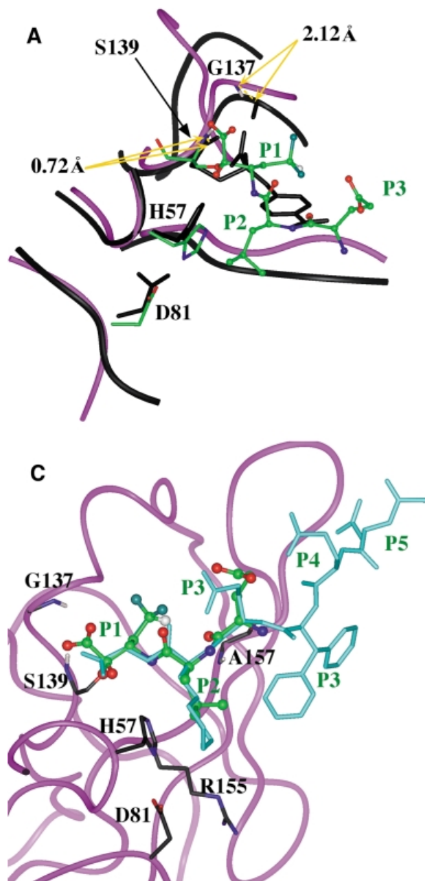
Fig. 5. (A) Expanded view of the pairwise superposition of the NS3-inhibitor complex S configuration (average minimized structure backbone in magenta ribbon, the catalytic triad in stick representation and the ketoacid inhibitor in ball-and-stick representation with atom type colour code) and APPA-trypsin complex (PDB accession code 1tpp, backbone in black ribbon and inhibitor in black stick representation), the SCR residues' backbone atoms have been used for the superposition. The resulting distances between equivalent nitrogen atoms forming the oxyanion hole are shown. (B) Pairwise superposition of the average minimized structures of the free enzyme, blue (PDB accession code 1bt7), and the complex, assuming the S configuration, magenta, with the inhibitor shown in ball-and-stick representation (green). The catalytic triad is reported in stick representation. The HN groups forming the oxyanion hole and their distances in the two structures are shown. The SCR strands that account mostly for the total r.m.s.d. observed (1.05 Å) are A2 and C2. (C) Pairwise superposition of the minimized average structure of the set assuming the S configuration, with inhibitor I in cyan stick representation (product of reaction inhibitor complex) (Cicero et al. , 1999). The backbone heavy atoms of the P1–P3 residues have been used in the superposition.
