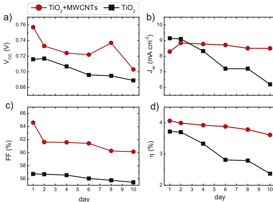
Fig. 5. Time dependence of the figures of merit of DSSCs with and without MWCNTs in the TiO 2 layer, under prolonged ambient light irradiation: (a) V_{oc} , (b) J_{sc} , (c) FF, and (d) \eta .
