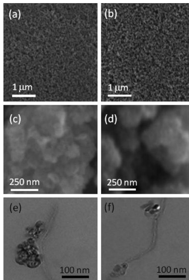
Fig. 1. SEM image at 10 kV of TiO 2 nanoparticle layer prepared in this work (a) without MWCNTs and (b) with 0.03% wt. MWCNTs; high magnification SEM image of TiO 2 nanoparticles (c) without MWCNTs and (d) 1.0% wt. MWCNTs. (e) TEM bright field image of TiO 2 agglomerates of nanoparticles connected to a MWCNT and (f) TEM bright field image of TiO 2 agglomerates associated to different sites of a MWCNT. Samples (e) and (f) make use of the same ratio of MWCNTs/TiO 2 (0.03% wt. of MWCNTs) and the TEM images were made at 200 kV.
