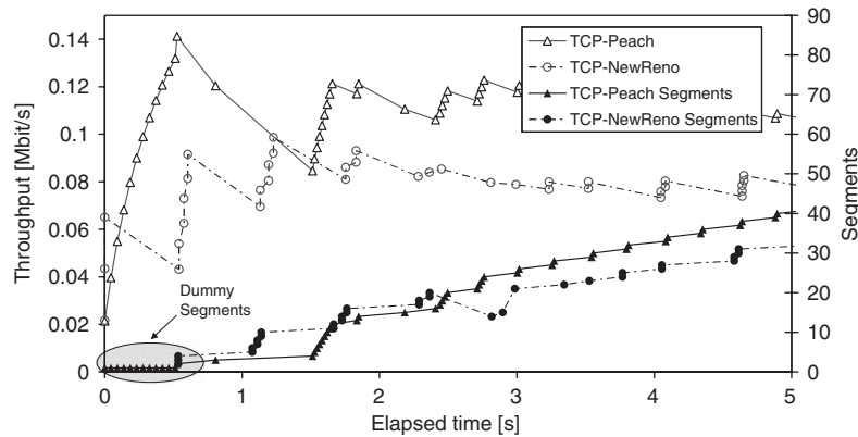
Figure 2. TCP Peach behaviour; RTT = 520 ms, PER = 1%, channel capacity = 2 Mbit/s, TCP segment size = 1448 bytes, gateway buffer size = bandwidth-delay product.
