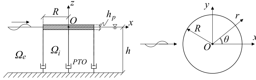
Fig. 1. View from above and horizontal cross-section of the flexible circular WEC.
