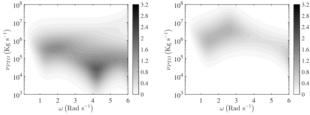
Fig. 2. Behaviour of C_W versus frequency of the incident waves \omega and PTO-Coefficient \nu_{PTO} . (a) 5 PTO devices located in r = 0 and r_i = R, \theta_i = [0, \pi/2, \pi, 3\pi/2] rad. (b) Single PTO device located at the centre of the plate.
