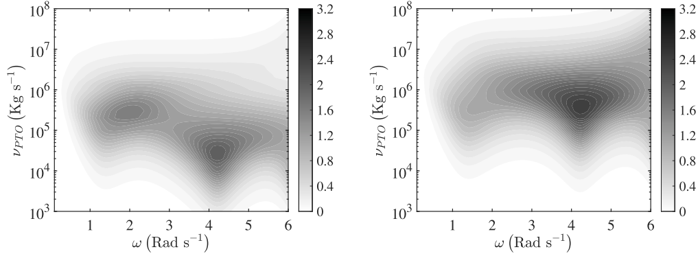
Fig. 3. Behaviour of C_W versus frequency of the incident waves and PTO-Coefficient. (a) PTO system characterised by a single PTO device in r = 0 and 8 PTO devices equally spaced in r = R ; (b) The case of 5 PTO devices located in r = 0 and r_i = R/2, \theta_i = [0, \pi/2, \pi, 3\pi/2] rad.
