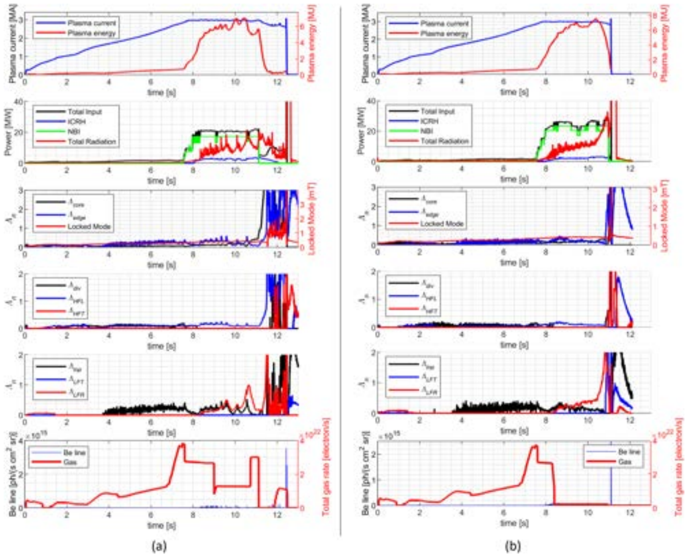
FIG. 9. Pulses 94 447 (a) and 94 655 (b): time traces of the plasma current and plasma energy (first row); input power and radiated power (second row); locked-mode amplitude and dimensionless core radiation factor (third row); dimensionless divertor, HFL, and HFT radiation factors (fourth row); dimensionless top, LFR, and LFT radiation factors (fifth row); outer Be II photon flux (used to detect ELMs) and total gas rate (sixth row). The right column shows the same plots with a zoom near the disruption.
