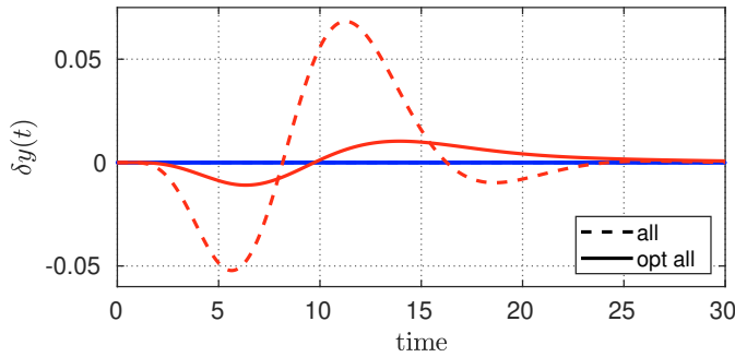
Fig. 6. Output variation \delta y(t) of the closed loop system with a non-optimized Allocator (dashed), and with the optimized Allocator (solid), with respect to the original closed-loop system; in blue the signals of the nominal plant and in red the signals of a perturbed plant.
