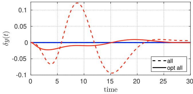
Fig. 4. Output variation \delta y(t) of the closed loop system with a non-optimized Allocator (dashed), and with the optimized Allocator (solid), with respect to the original closed-loop system; in blue the signals of the nominal plant and in red the signals of a perturbed plant.
