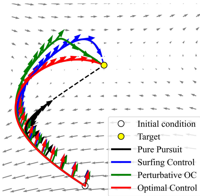
Fig. 6 Control strategies in a simple 2d flow. Trajectories obtained in a 2-dimensional steady linear flow. Pure Pursuit strategy (black), Surfing Control (blue), Perturbative Optimal Control (green) and Optimal Control (red). The trajectories are shown in the relative coordinate space, \mathbf{R} = (R_x, R_y) , thus the target is fixed in the origin (full yellow circle). The dashed lines show the trajectories followed by the strategies after the capture time of OC. The arrows indicate the control directions followed by each strategy.
