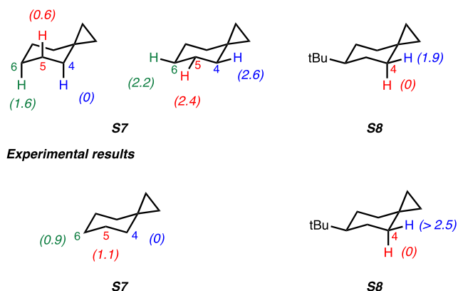
Figure 6. Difference in activation free energies ( \Delta\Delta G^\ddagger , in kcal mol -1 ) for HAT from the C–H bonds of S7 and S8 to ETFDO: computational and experimental studies.
