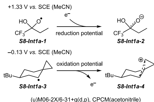
Figure 9. (a) Charge distribution of S8-Int1 by CMS and the electrostatic potential on a constant electron density surface. The regions of positive and negative potential are indicated in blue and red. (b) Spin density of the hypothetical triplet radical pair S8-Int1a . (c) In silico redox potentials of 1,1,1-trifluoro-2-hydroxybutoxy and 6-( tert -butyl)spiro[2.5]octan-4-yl radicals.
