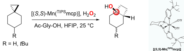
Scheme 1. Results Obtained in the Oxidation of Spiro[2.5]octanes with H 2 O 2 Catalyzed by [(S,S)-Mn( TIPS mcp)] (HFIP = 1,1,1,3,3,3-Hexafluoro-2-propanol)
