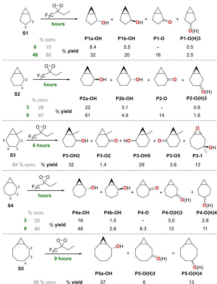
Scheme 3. Oxygenation of Bicyclo[ n .1.0]alkanes ( n = 3–6) (S1–S5) Promoted by ETFDO
