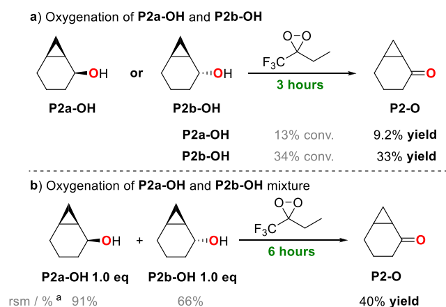
Scheme 5. Oxygenation of cis -Bicyclo[4.1.0]heptan-2-ol (P2a-OH) and trans -Bicyclo[4.1.0]heptan-2-ol (P2b-OH) a
