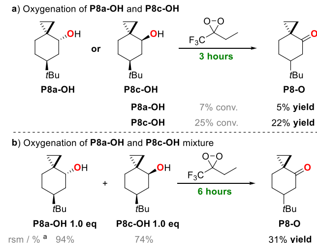
Scheme 6. Oxygenation of trans -6- tert -Butylspiro[2.5]octan-2-ol (P8a-OH) and cis -6- tert -Butylspiro[2.5]octan-2-ol (P8c-OH) a
