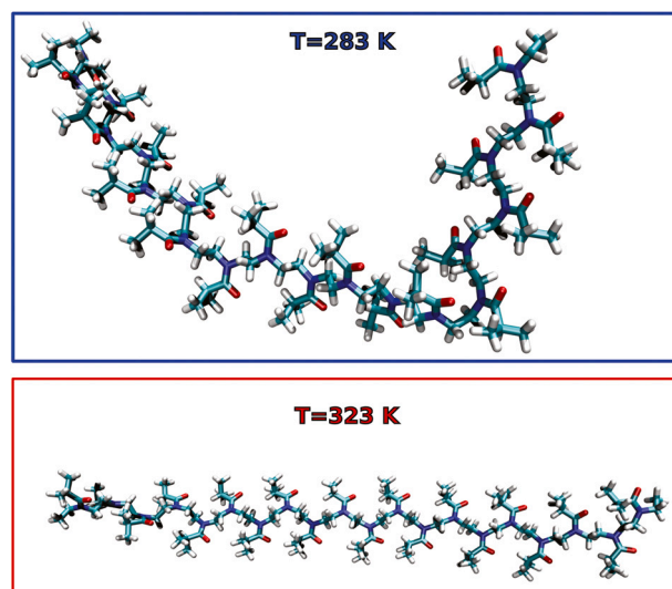
Fig. 4. Representative snapshots extracted from the aqueous PiPOx20 simulations at T = 283 K and T = 323 K. While in the former case the polymer average conformation is slightly folded, the macromolecular chain at high temperature is steadily stretched into all-trans conformations. A periodicity of 6.5 \text{ \AA} is obtained for the high-temperature conformation, in line with the X-ray data measured from the polymer crystals.
