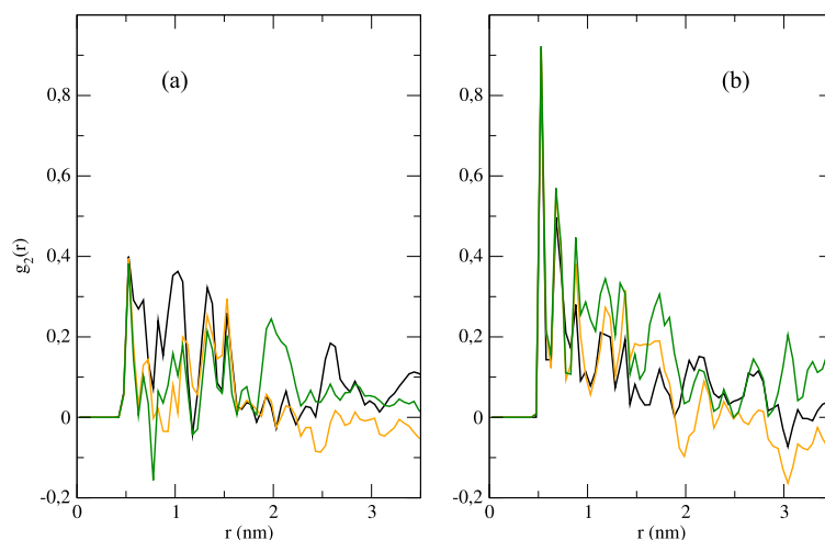
Fig. 7. Panel (a): low temperature g_2(r) for the three axes ( g_{2aa}(r) , g_{2bb}(r) and g_{2cc} , green, orange and black lines, respectively). Panel (b) high temperature g_{2aa}(r) , g_{2bb}(r) and g_{2cc} (green, orange and black lines, respectively). A first pronounced peak is appreciable for the system at high temperature.
