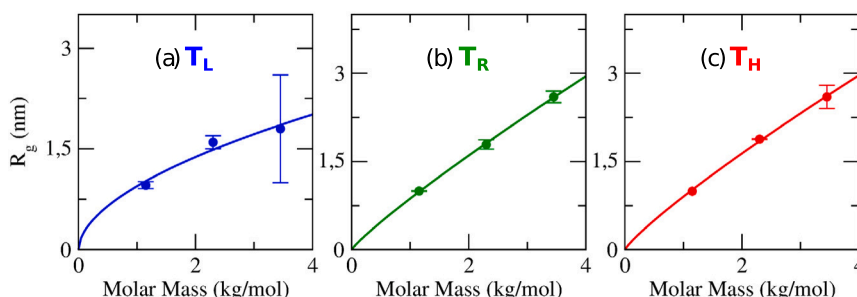
Fig. 2. Radius of gyration ( R_g ) of PiPOx as a function of the polymer molar mass for the single molecule aqueous solutions below the T_{cp} , at room temperature and above the T_{cp} (i.e., T = T_L = 283 K, T = T_R = 303 K and T = T_H = 323 K, respectively). While the T_L systems grow with a power law as a function of the molar mass, the trend of R_g as a function of the polymer molar mass at high temperature is shown to grow almost linearly with the molar mass: at high temperature conditions every increase in repeating units leaves the chain unfolded (the fitting curves are reported as full lines in each plot).
