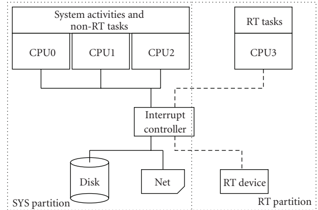
FIGURE 4: ASMP-Linux partitioning.
