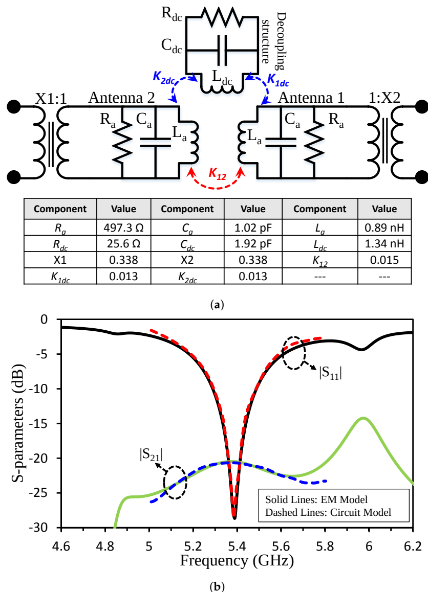
Figure 6. (a) Equivalent circuit model of the two-element MIMO antenna with decoupling structure, and (b) S-parameters comparison of the EM model (solid lines) and circuit model (dashed lines).
