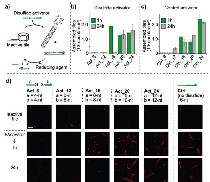
Figure 3. Transient self-assembly of DNA-based nanostructures driven by redox fuels. (a) Transient self-assembly induced by a disulfide activator achieved in the presence of a reducing agent. (b) Histograms of assembled tile density (assembled tile count/mm 2 ) measured from fluorescence microscopy images taken before and after (1 h and 24 h) the addition of disulfide activators of different lengths. (c) Same experiment as in panel a but using control activators lacking the disulfide bond. (d) Fluorescence microscope images obtained with the disulfide activators and one control activator (Ctrl 16 ). The experiments shown in this figure were performed in
