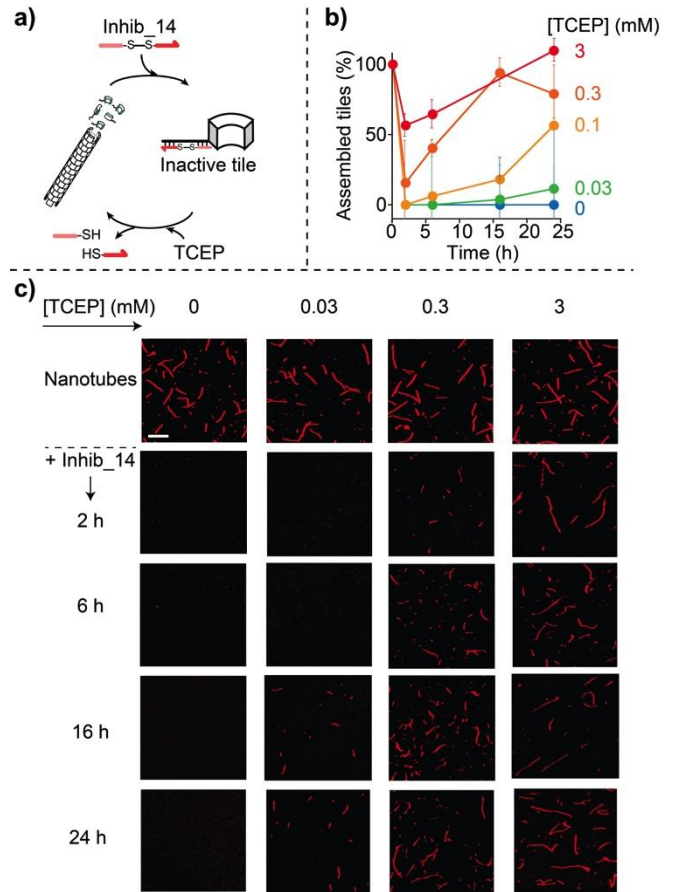
Figure 7. Modulation of the transient disassembly of DNA-based nanostructures. (a) Transient disassembly induced by a disulfide inhibitor can be modulated by varying the concentration of the reducing agent (TCEP). (b) Normalized assembled tile density (assembled tile count/mm 2 , for nanotubes longer than 1 μm) measured from the fluorescence microscopy images obtained before and after (2, 6, 16 and 24 h) the addition of the disulfide inhibitor (Inhib_14) in the presence of different concentrations of TCEP. The experiments shown in this figure were performed in 1 × TAE, 12.5 mM MgCl 2 at pH 8.0, 25 °C with different concentration of TCEP (indicated in the figure). Nanotube disassembly was carried out in the presence of nanotubes formed from active DNA tiles (500 nM) by adding the disulfide or the control inhibitor (1 μM). The experimental values represent averages of three separate measurements and the error bars reflect the standard deviations. Scale bars for all microscope images, 5 μm.
