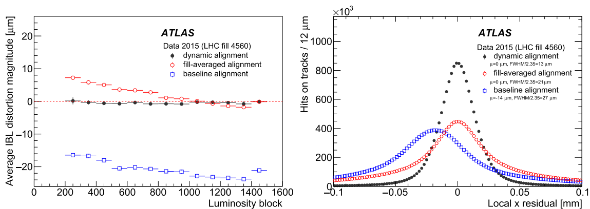
Fig. 11 IBL distortion magnitude in the transverse plane per luminosity block (LB) range (left) and the IBL local- x unbiased residual distributions (right) for an LHC fill averaged over all 14 IBL staves. The open blue squares (baseline alignment) show the average IBL dis-
