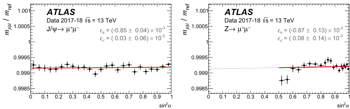
Fig. 22 Ratio of the measured mass to the reference as a function of \sin^2\alpha . Due to event kinematics, J/\psi \rightarrow \mu^+\mu^- events (left) cover the entire \sin^2\alpha range while Z \rightarrow \mu^+\mu^- events (right) cover a smaller
