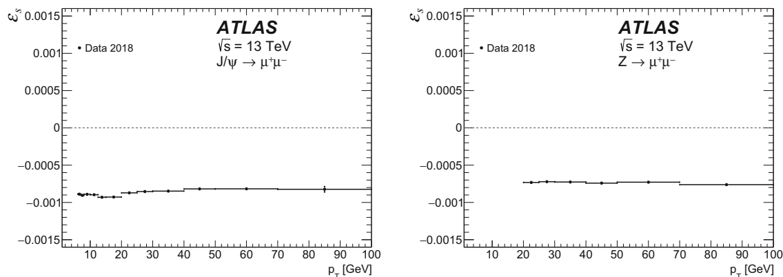
Fig. 23 The measured momentum scale bias \varepsilon_s as a function of track p_T . Error bars represent the statistical uncertainty. Left: J/\psi \rightarrow \mu^+\mu^- decays; right: Z \rightarrow \mu^+\mu^- decays
