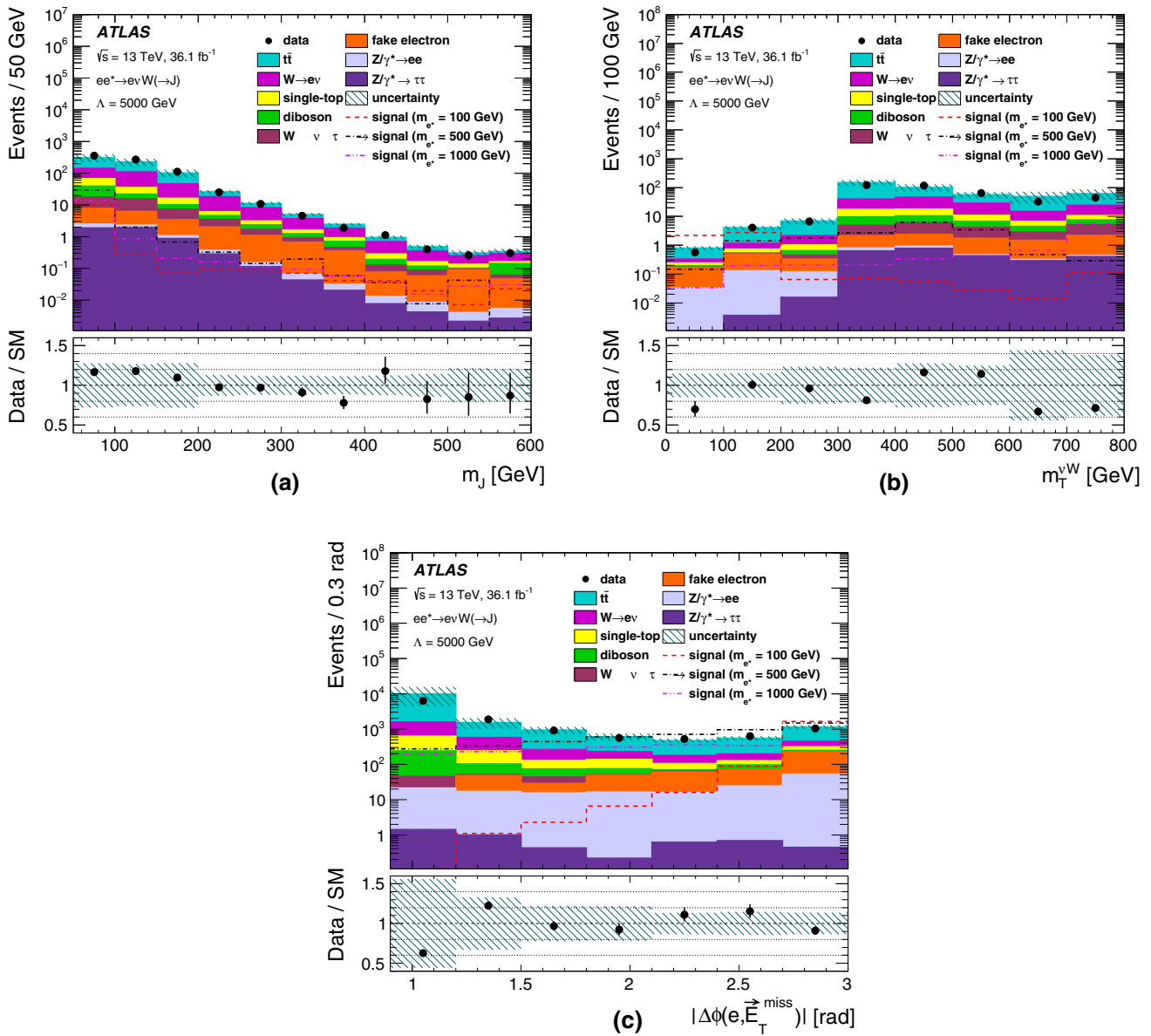
Fig. 4 The distributions of a m_J , b m_T^{\nu W} , and c |\Delta\phi(e, \vec{E}_T^{\text{miss}})| used to discriminate the signal and background processes in the e\nu J channel. The distributions are shown after applying the preselection criteria. The background contributions are constrained using the CRs. The signal models assume \Lambda = 5 TeV. The last bin includes overflow events
